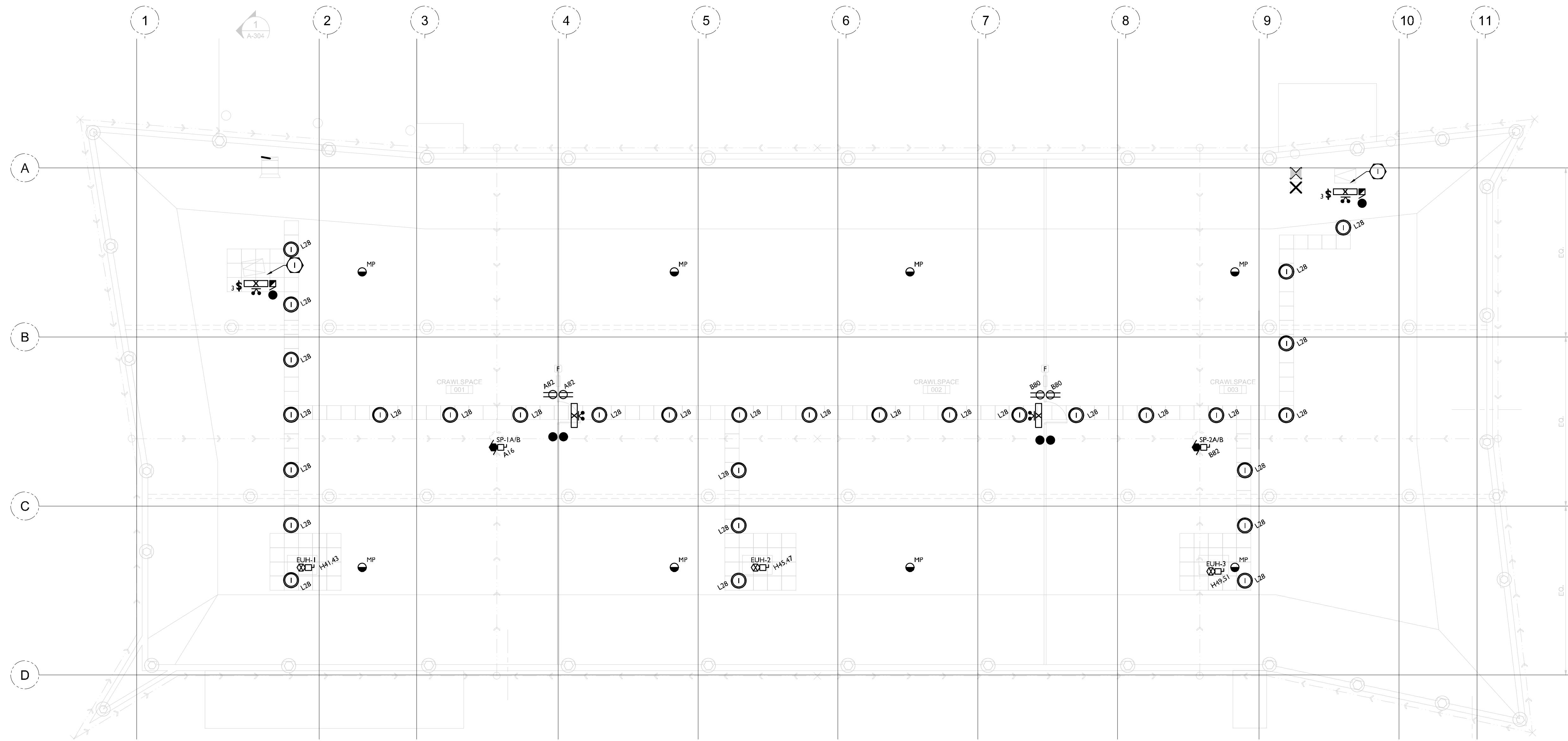
ELECTRICAL - CRAWLSPACE LAYOUT E-105 SCALE: 1:100
