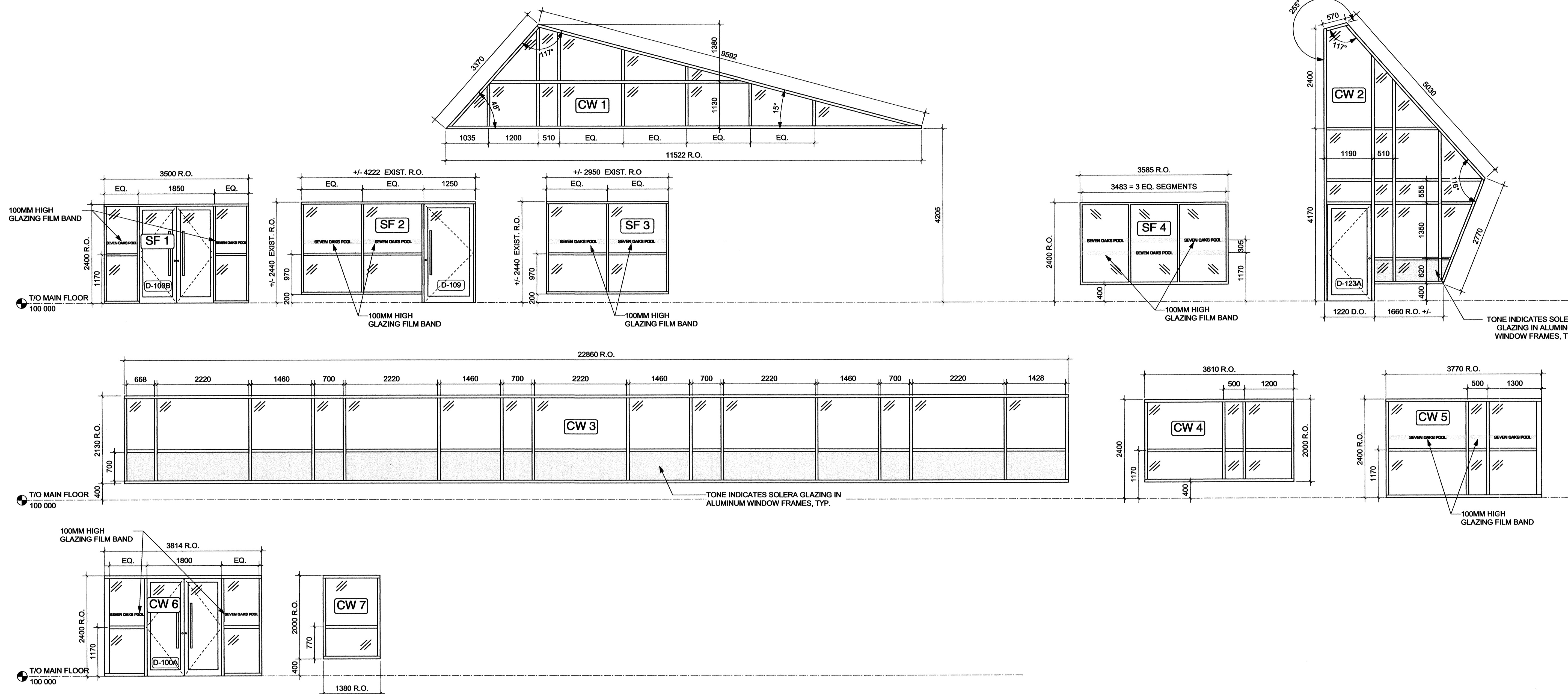
1 GLAZING SCHEDULE 1:50
