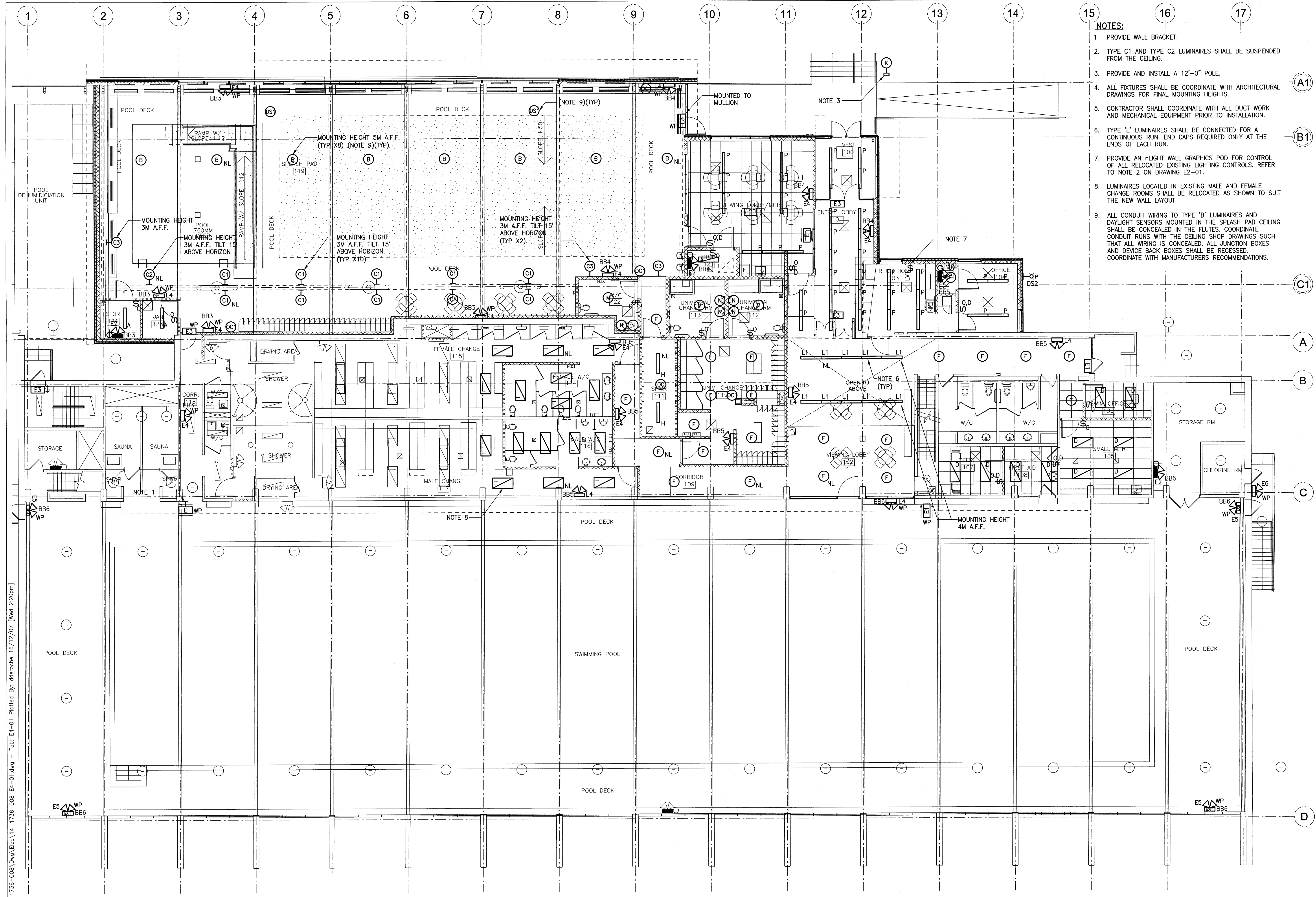
1 MAIN FLOOR LIGHTING PLAN - NEW SCALE: 1:100mm (24"x36")
