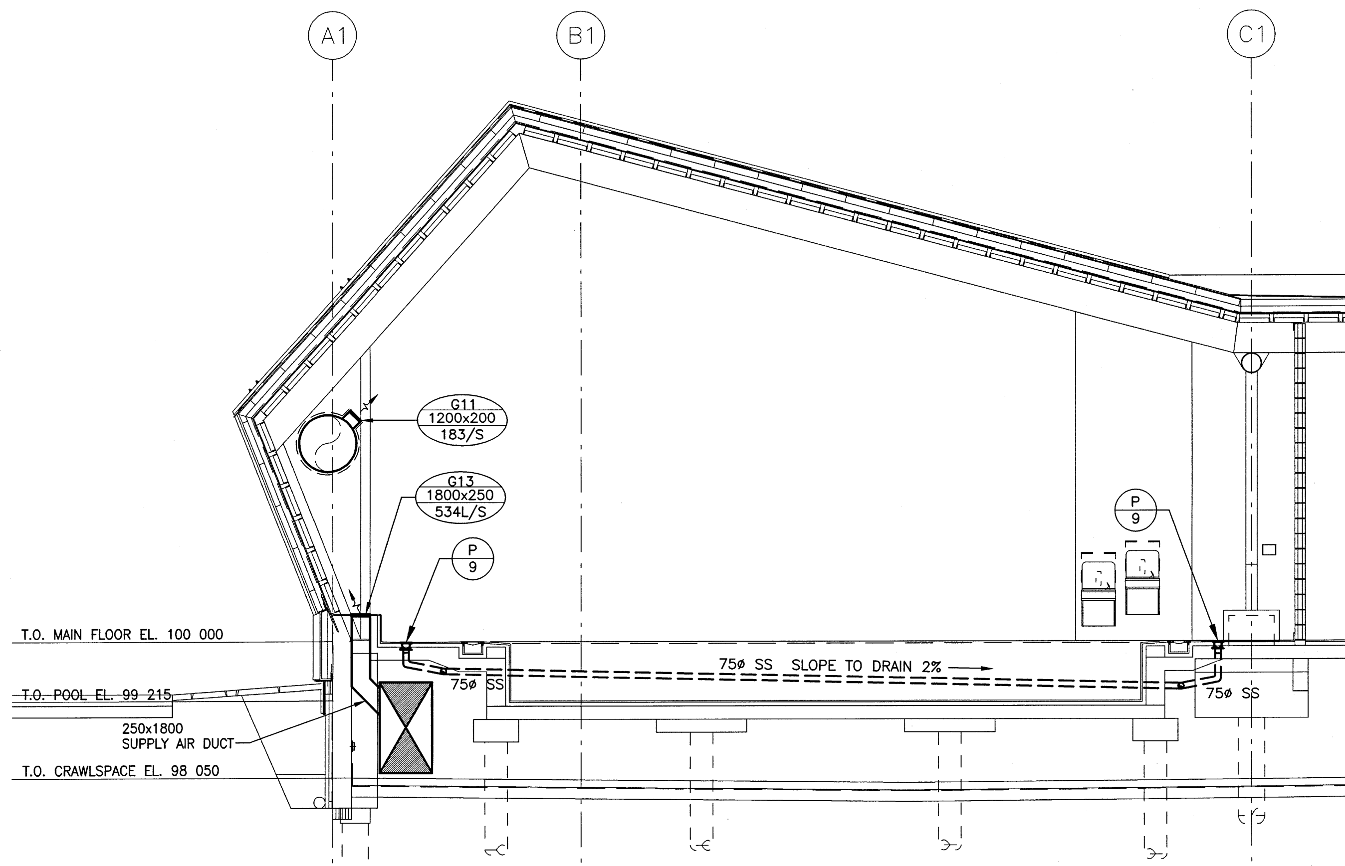
3 POOL DRAINS SANITARY PIPING DETAIL M2-01 SCALE: N.T.S.
