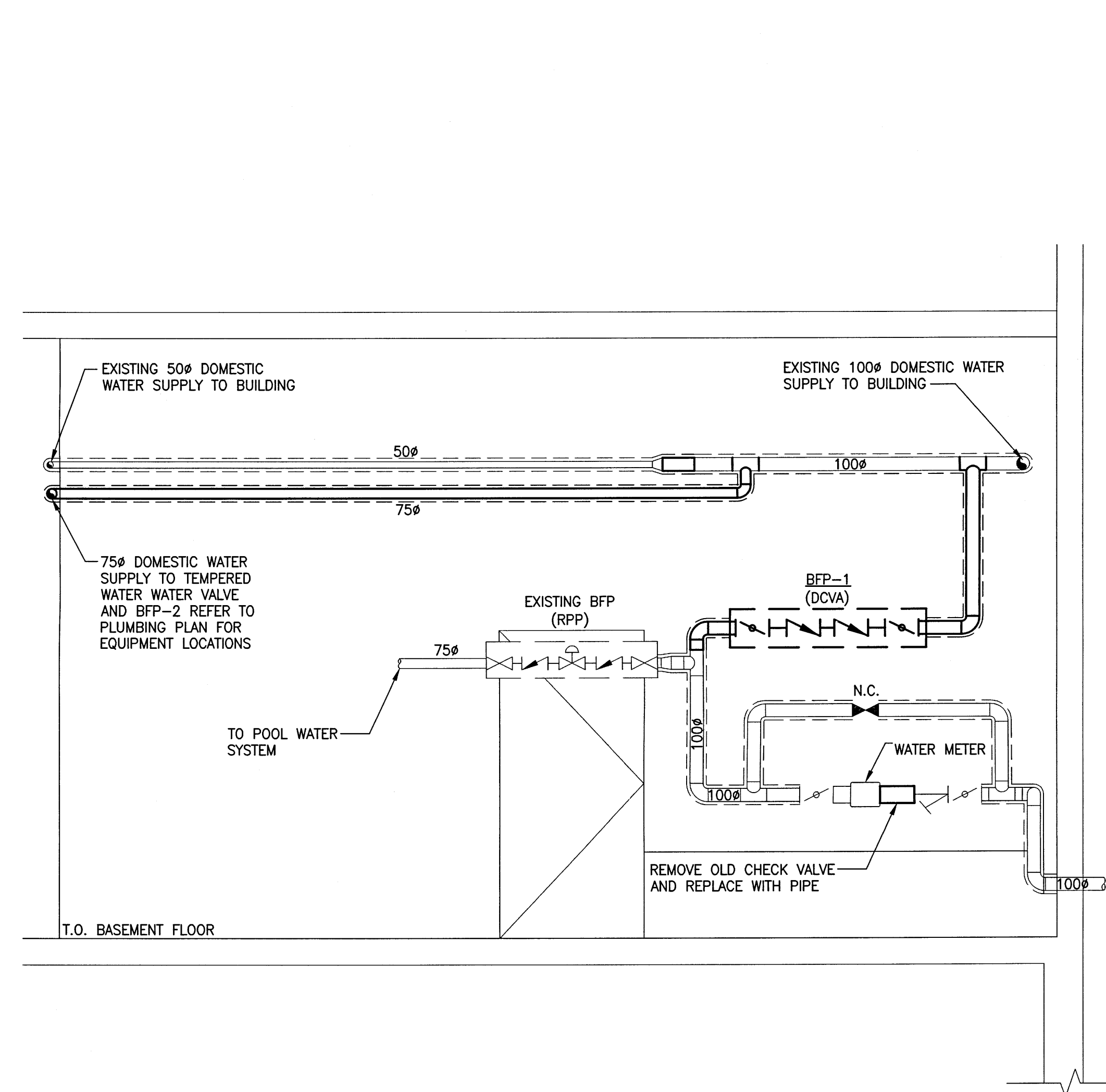
1 DOMESTIC WATER SERVICE ENTRANCE DETAIL M2-00 SCALE: N.T.S.
