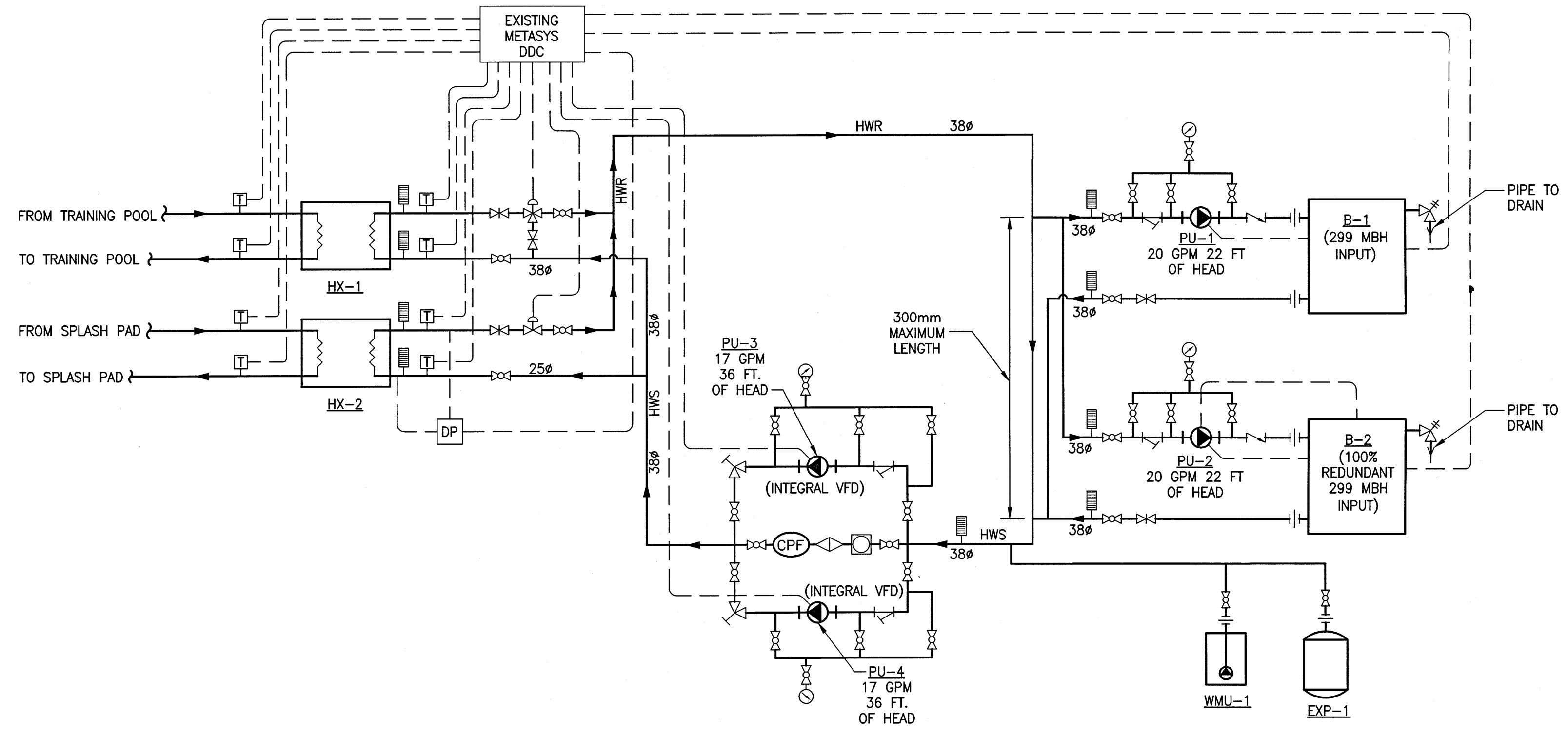
1 POOL WATER HEATING PIPING SCHEMATIC SCALE: N.T.S.
