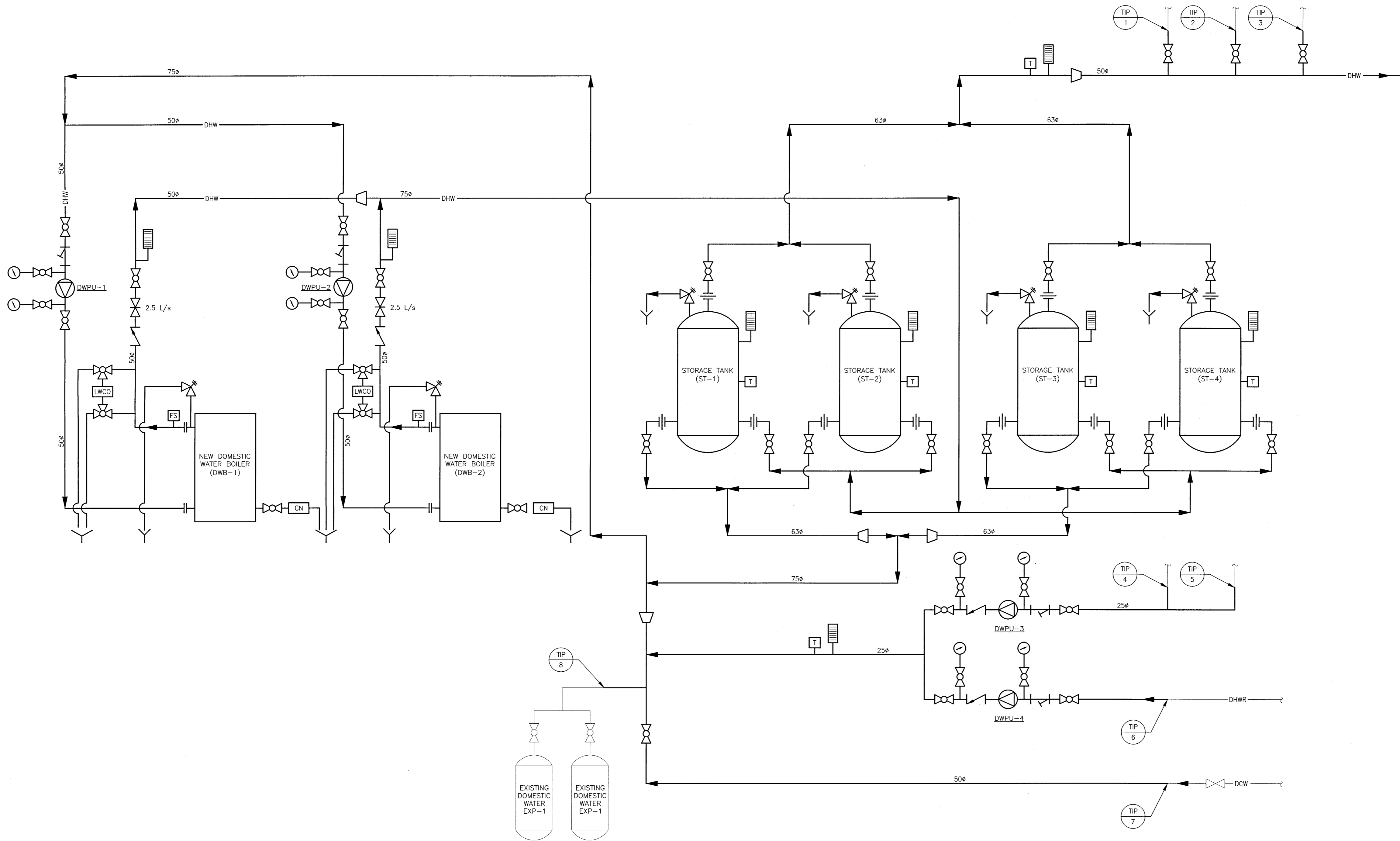
PIPING SCHEMATIC - NEW DOMESTIC WATER BOILERS AND STORAGE TANKS SCALE N.T.S.
