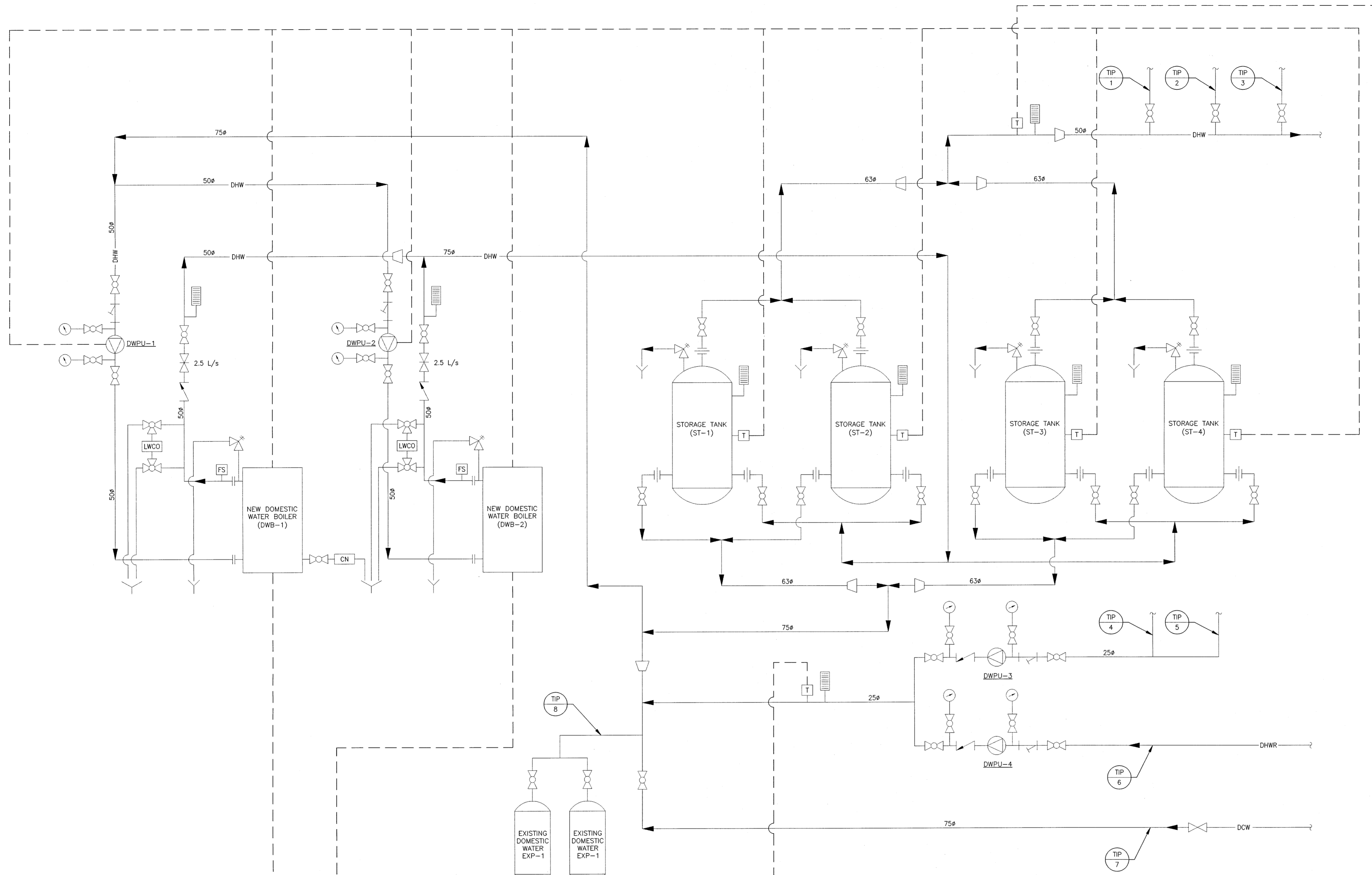
CONTROLS SCHEMATIC - NEW DOMESTIC WATER BOILERS AND STORAGE TANKS SCALE N.T.S.
