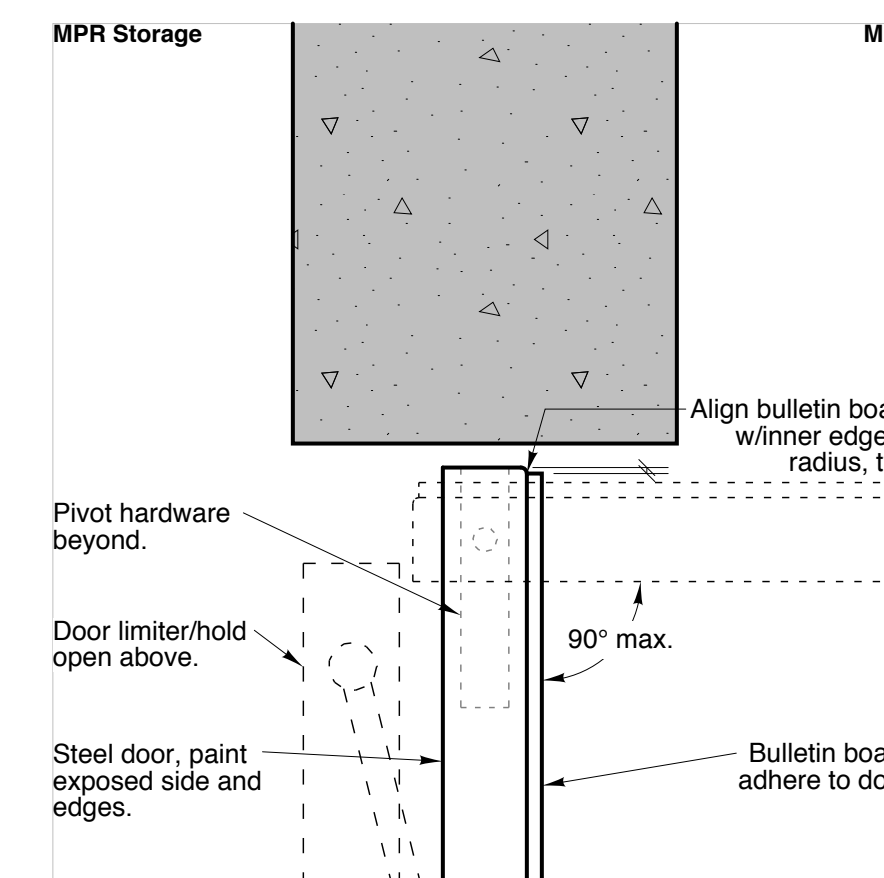
14 plan detail a503 3"=1'-0"
