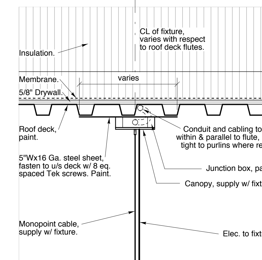
15 section detail a503 1 1/2"=1'-0"
