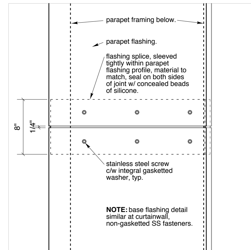
8 plan detail a503 1 1/2"=1'-0"
