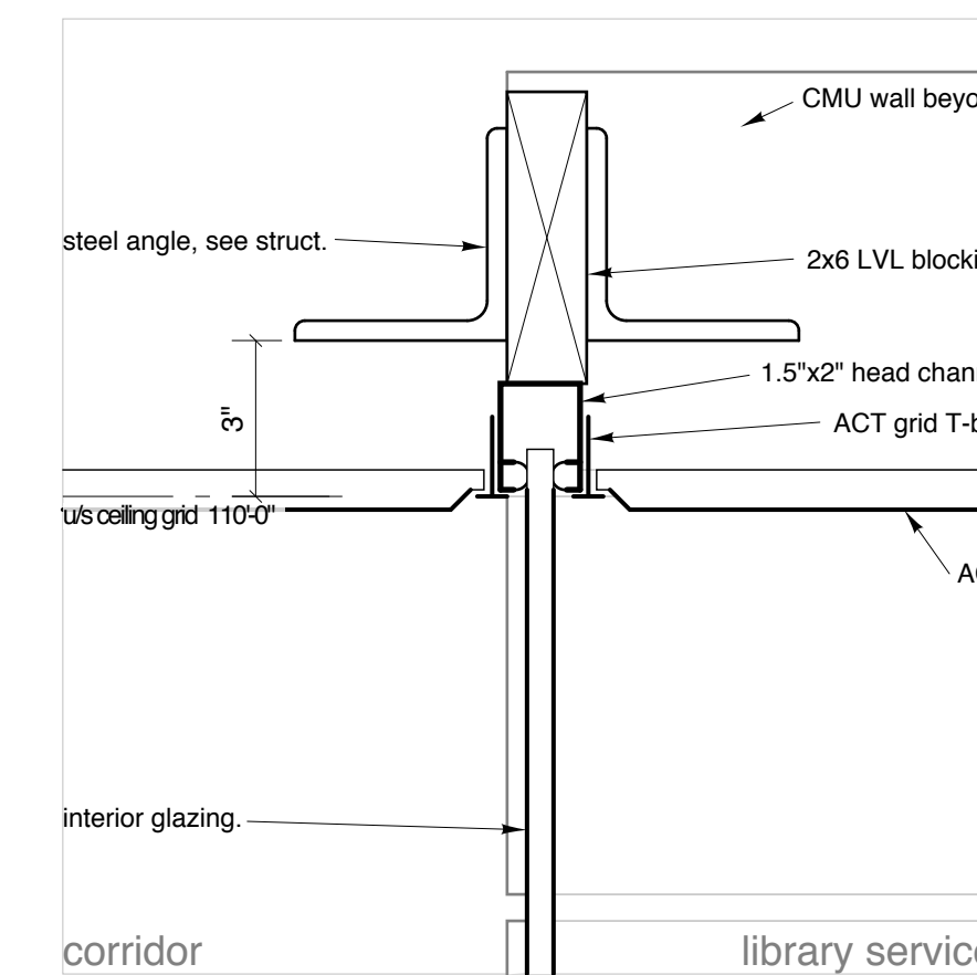
5 section detail a503 3"=1'-0"
