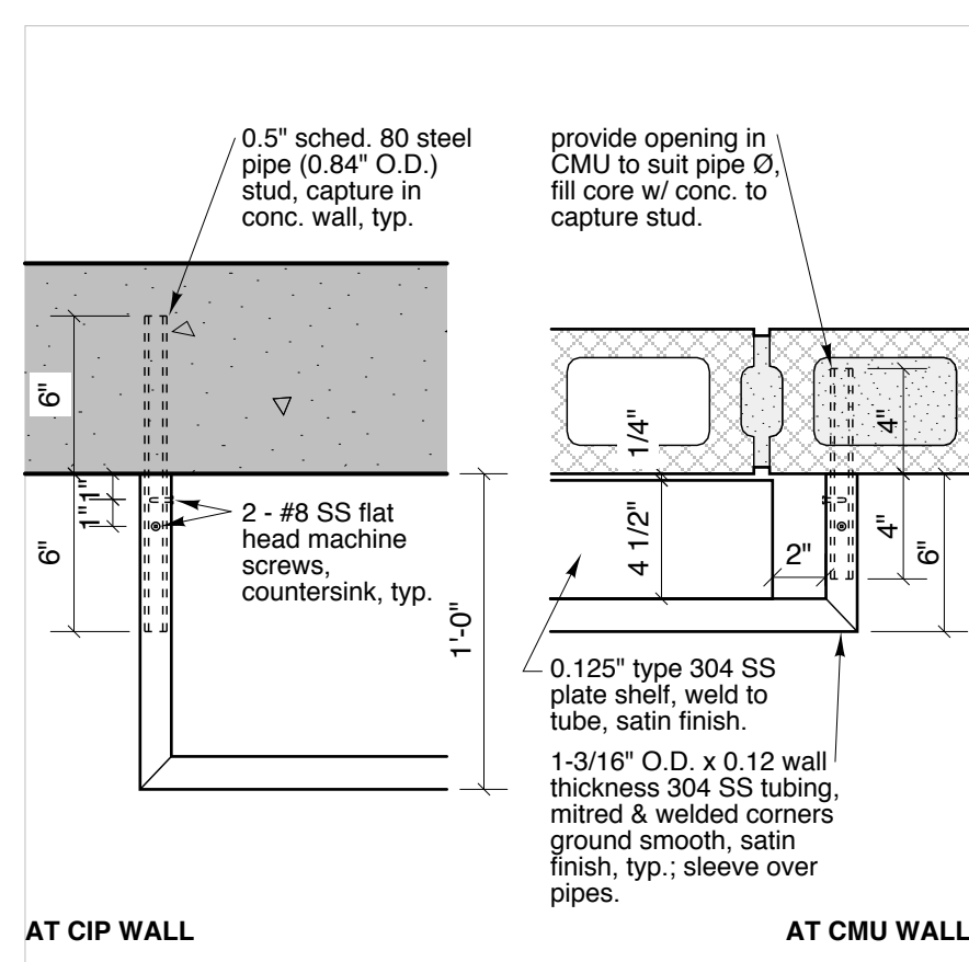
11 plan detail a503 1 1/2"=1'-0"
