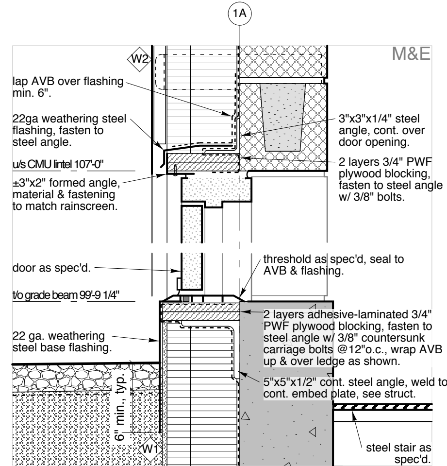
2 section detail a503 1 1/2"=1'-0"
