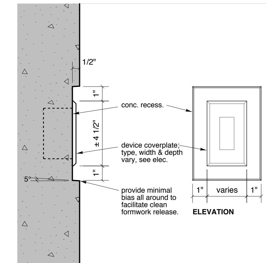
10 section detail a503 3"=1'-0"
