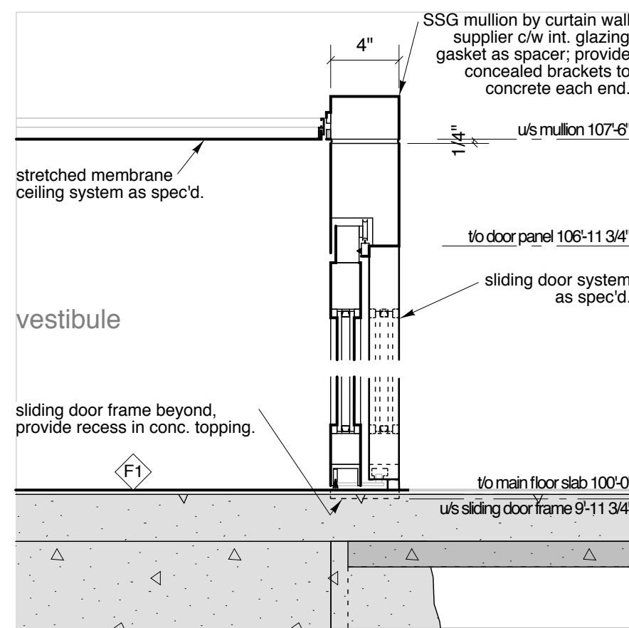
1 section detail a503 1 1/2"=1'-0"
