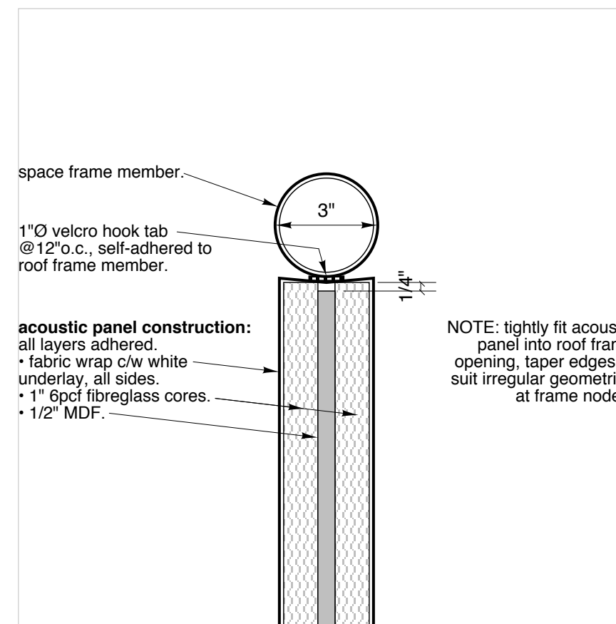
7 section detail a503 3"=1'-0"
