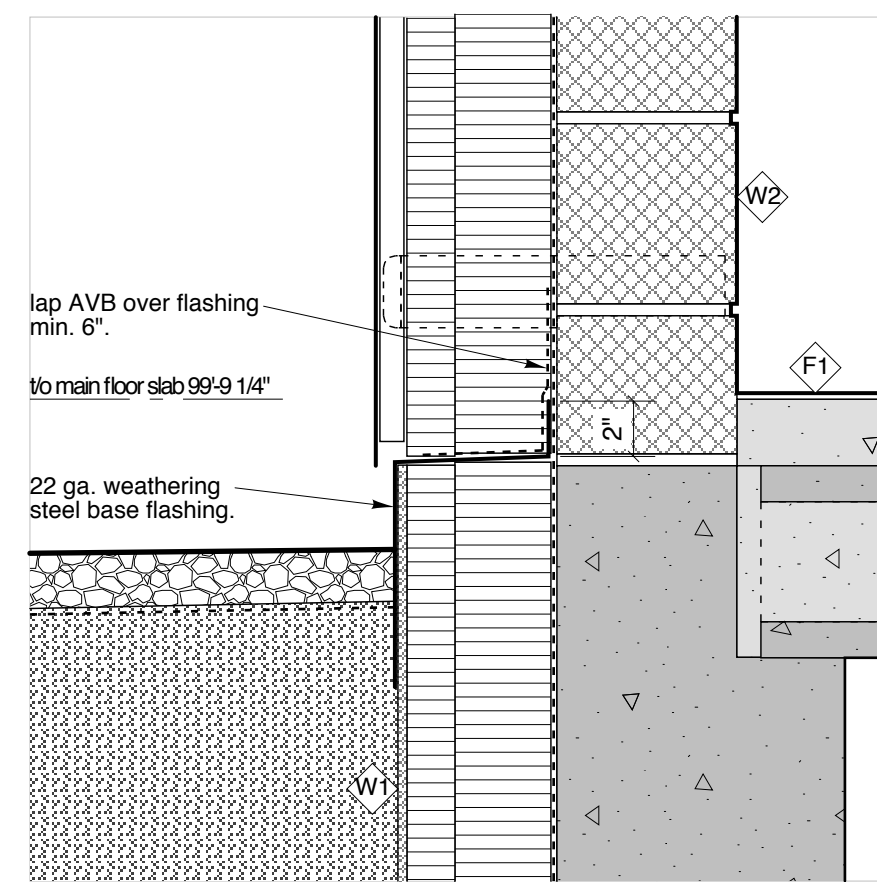
3 section detail a503 1 1/2"=1'-0"
