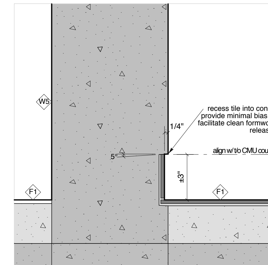
9 section detail a503 3"=1'-0"
