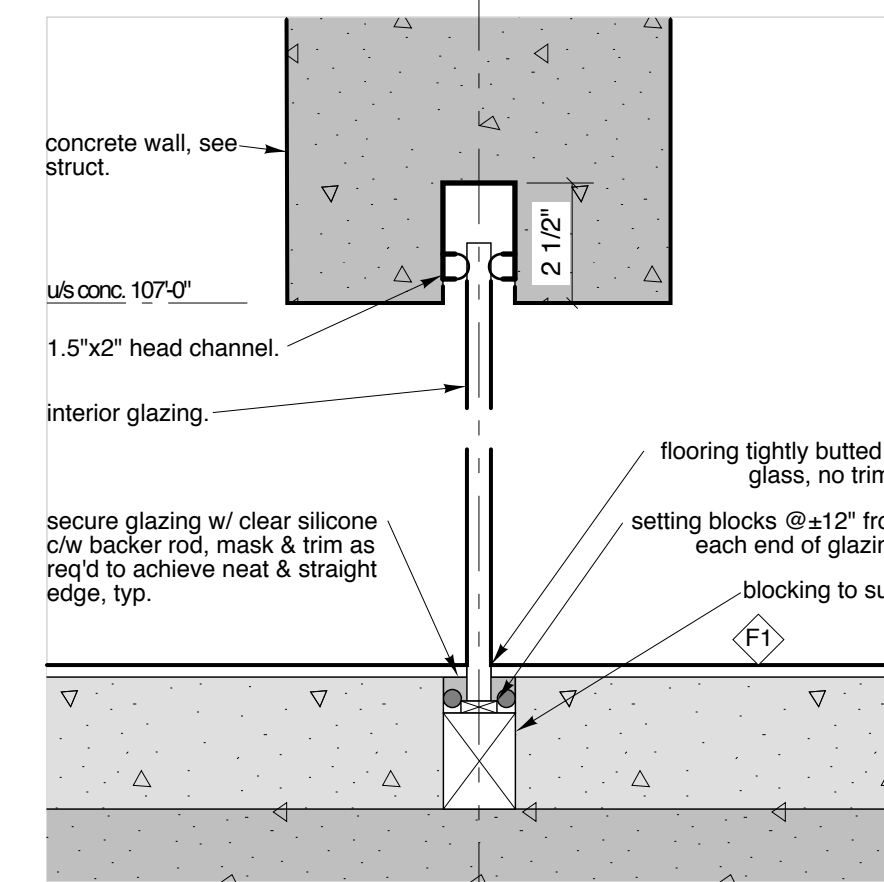
4 section detail a503 3"=1'-0"
