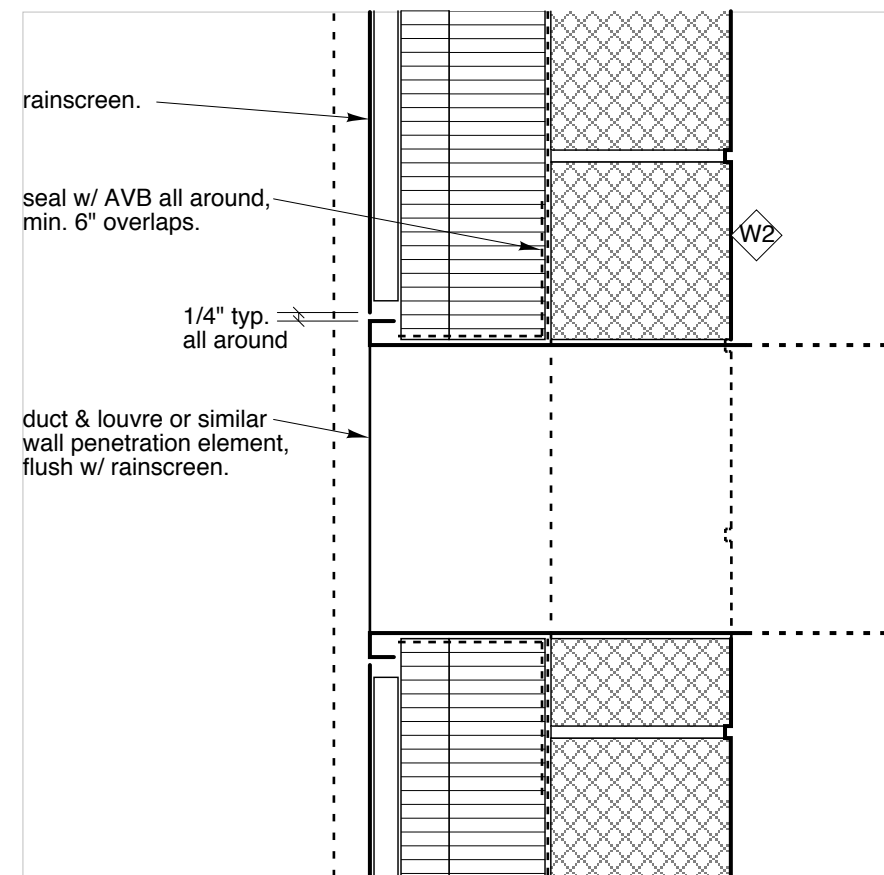
6 section detail a503 1 1/2"=1'-0"
