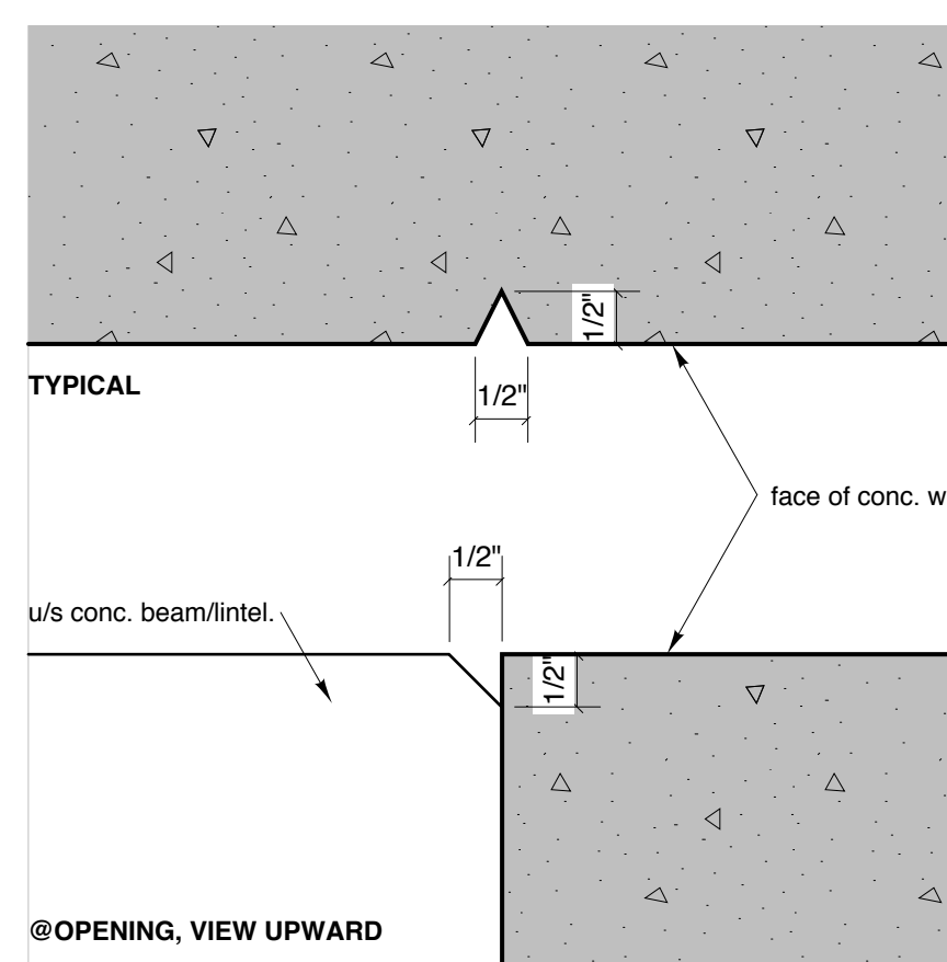
12 section detail a503 6"=1'-0"
