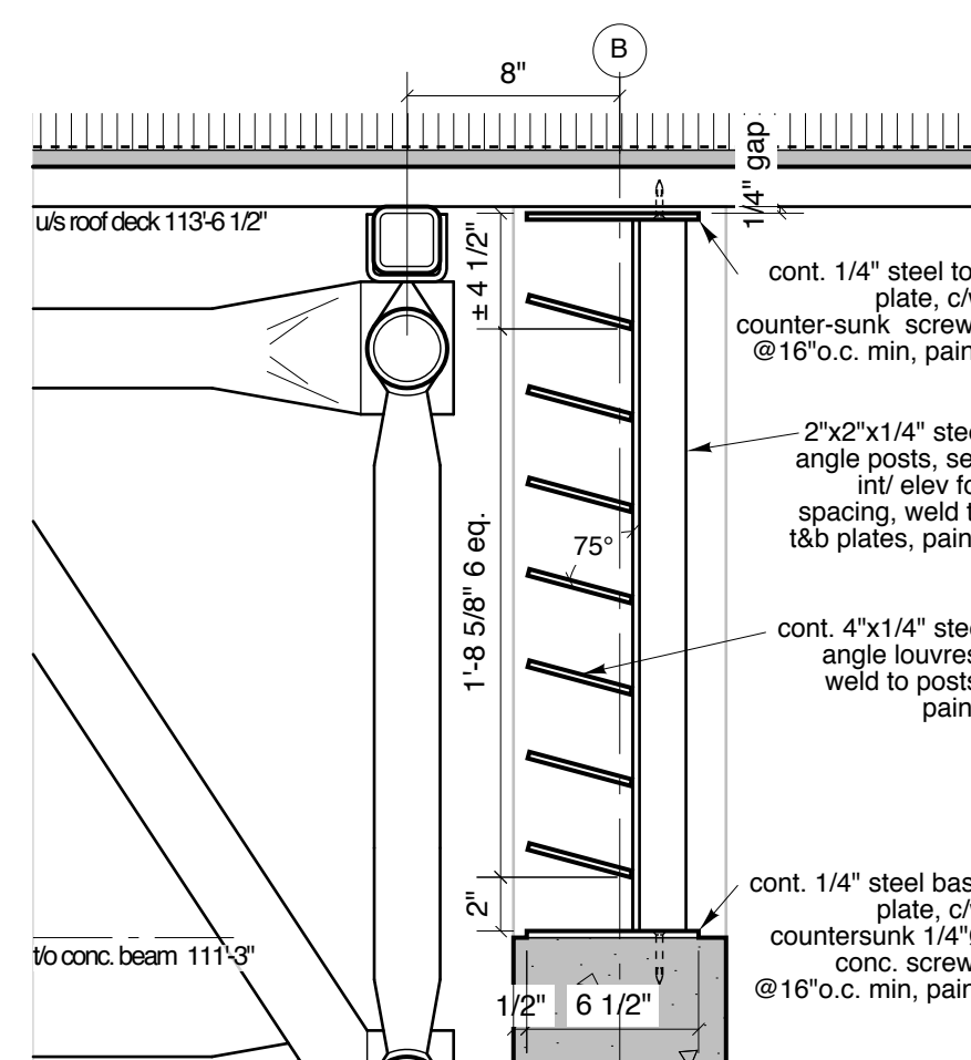
13 section detail a503 1 1/2"=1'-0"
