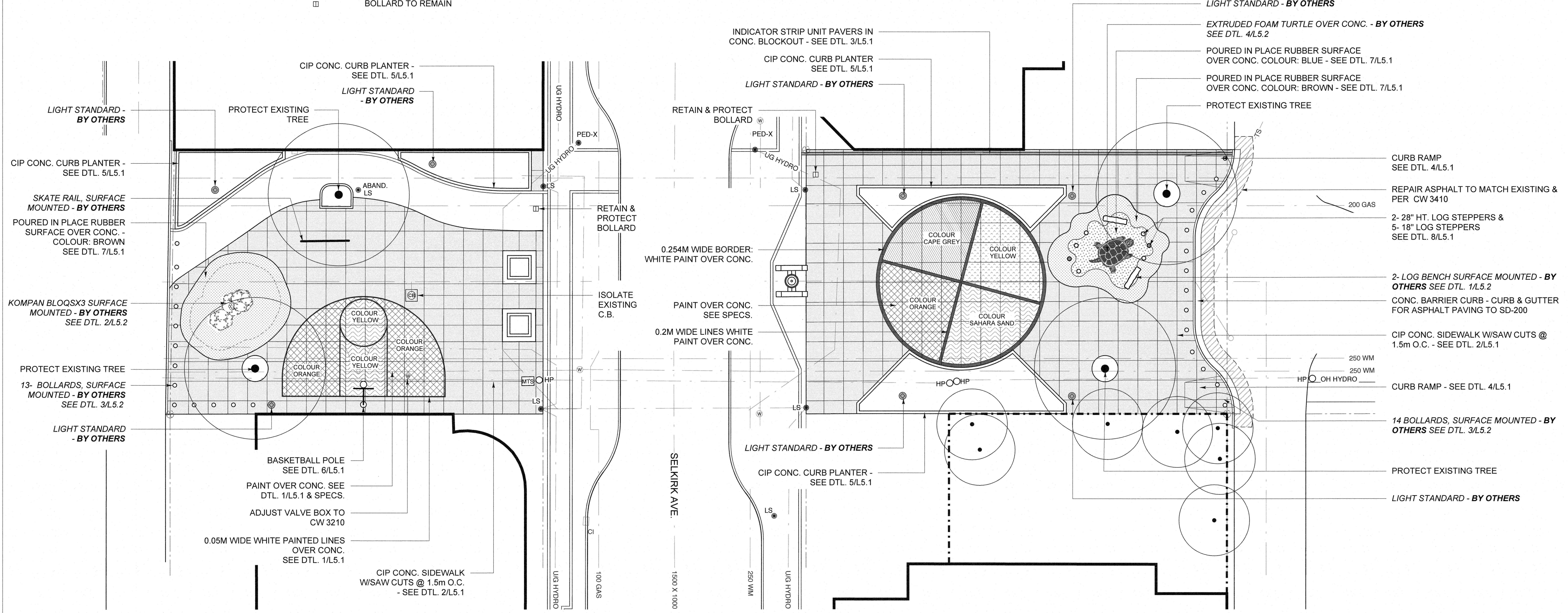
1 MATERIALS PLAN L4.0 SCALE: 1:150
