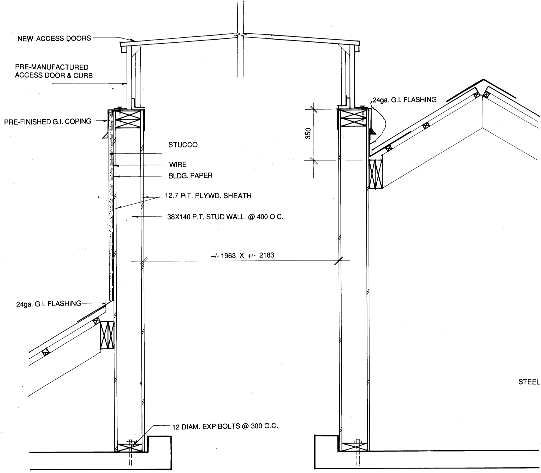
4 DETAIL THROUGH ACCESS HATCH SCALE -- 1:10
