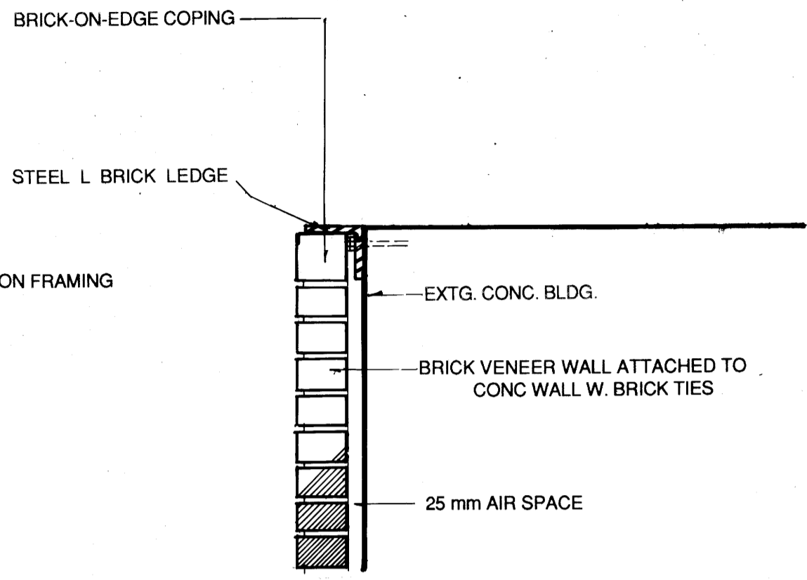
3 SECTION DETAIL : BRICK COPING SCALE -- 1:10
