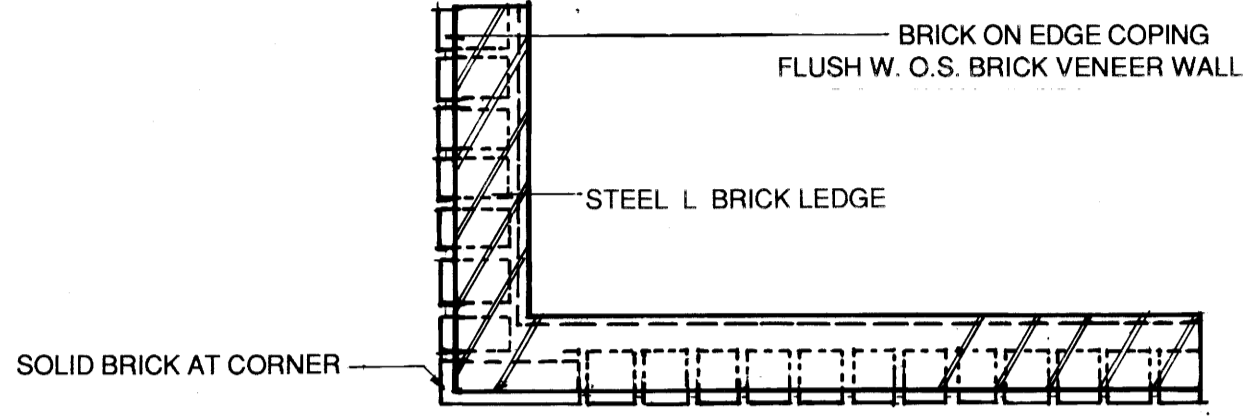
5 PLAN DETAIL : BRICK COPING SCALE -- 1:10
