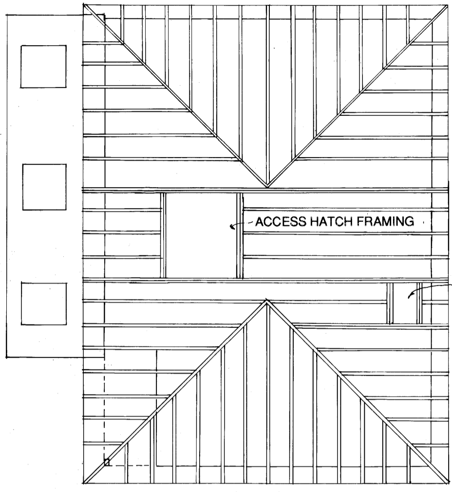
1 ROOF FRAMING PLAN SCALE -- 1:100
