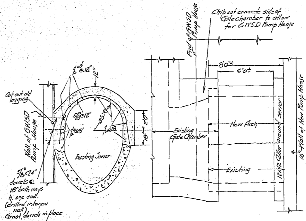
Revised Repairs to Arch of Existing Sewer Scale 1/4" = 1' foot
