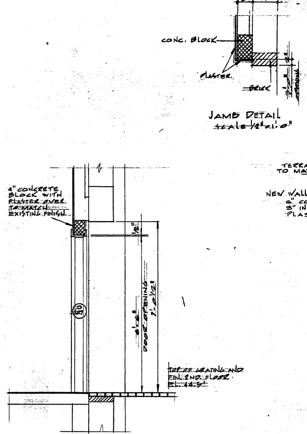
SECTION 13C SCALE 1/2" = 1'-0"
