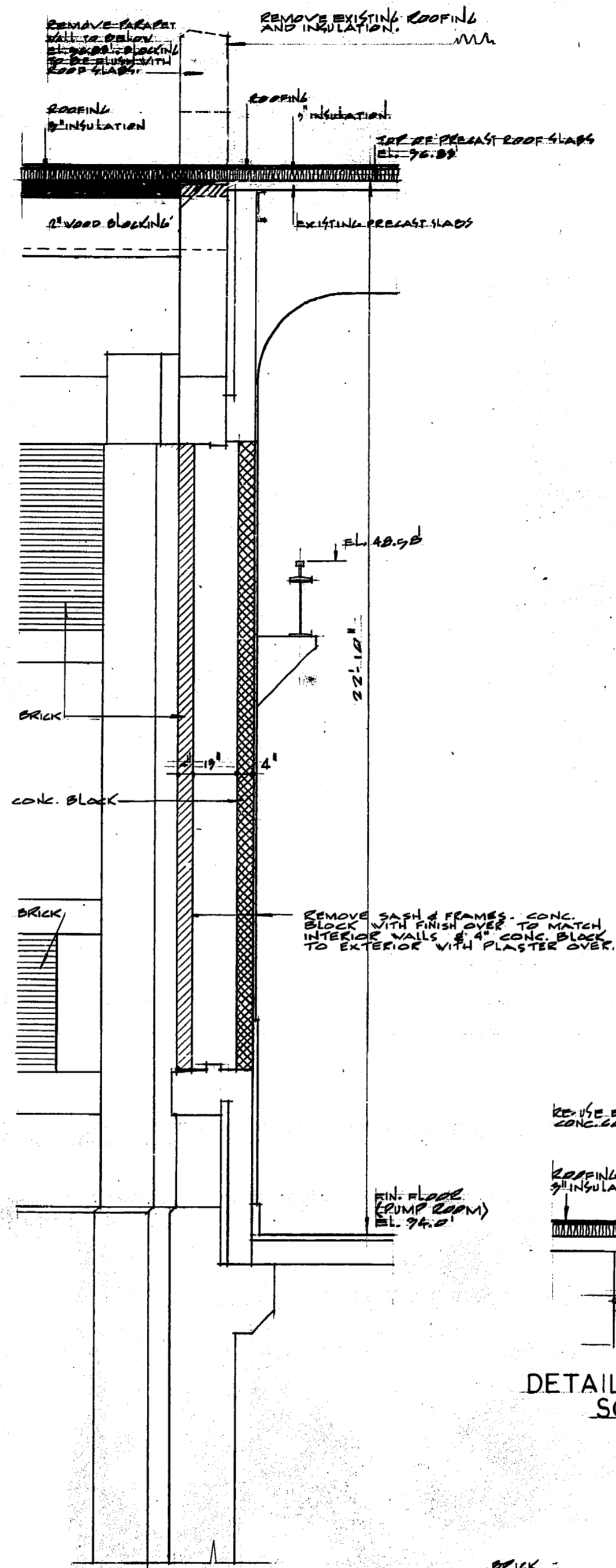
SECTION 13B SCALE 1/2" = 1'-0"
