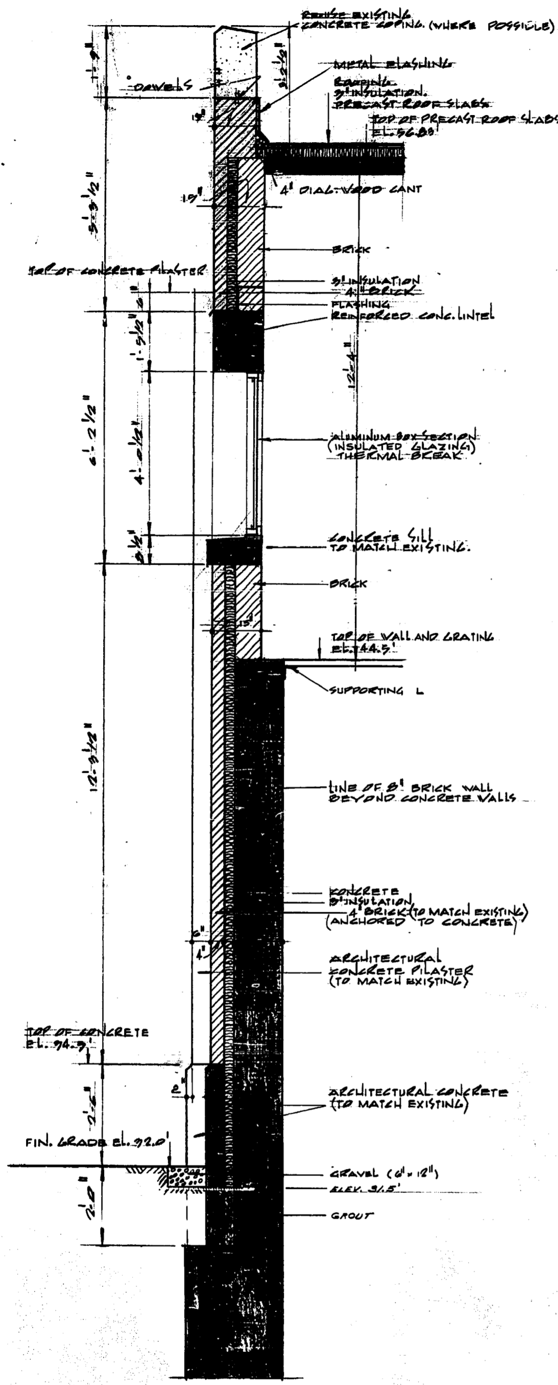
SECTION 13A SCALE 1/2" = 1'-0"
