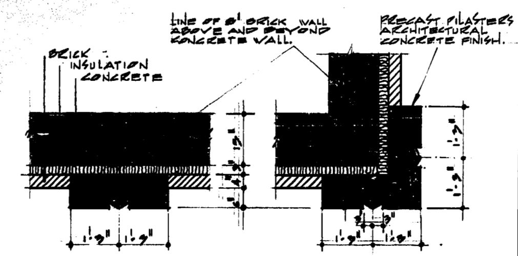
TYPICAL CONCRETE PILASTER DETAILS SCALE 1/2" = 1'-0" FOR ACTUAL ELEV. SUBTRACT 0.37 FT.
