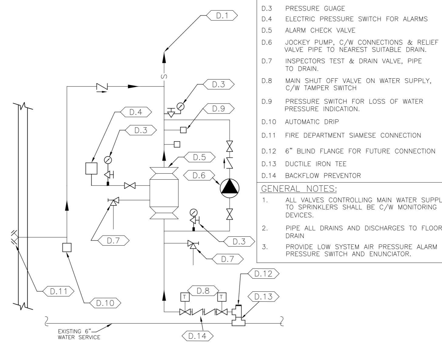
4 WET SYSTEM SPRINKLER TREE SCHEMATIC
