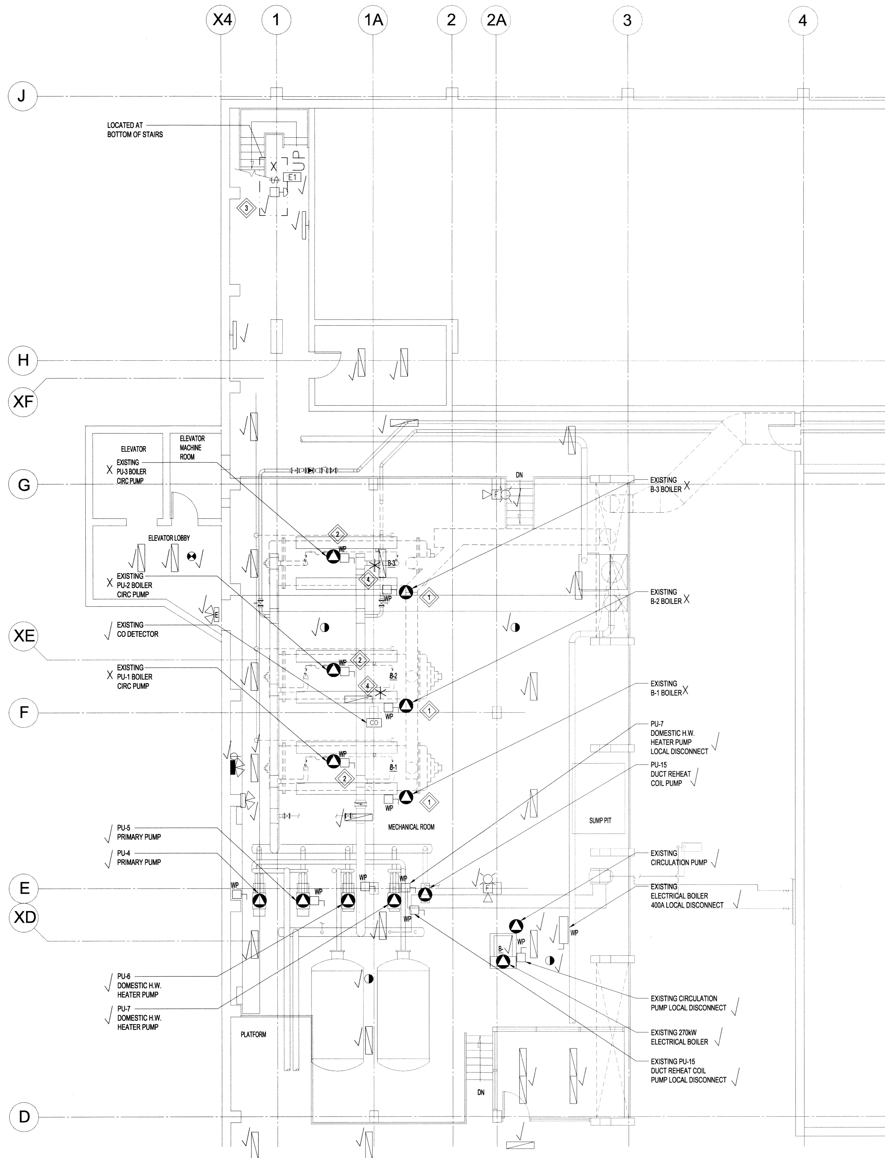
BOILER ROOM PLAN - DEMO SCALE 1:75
