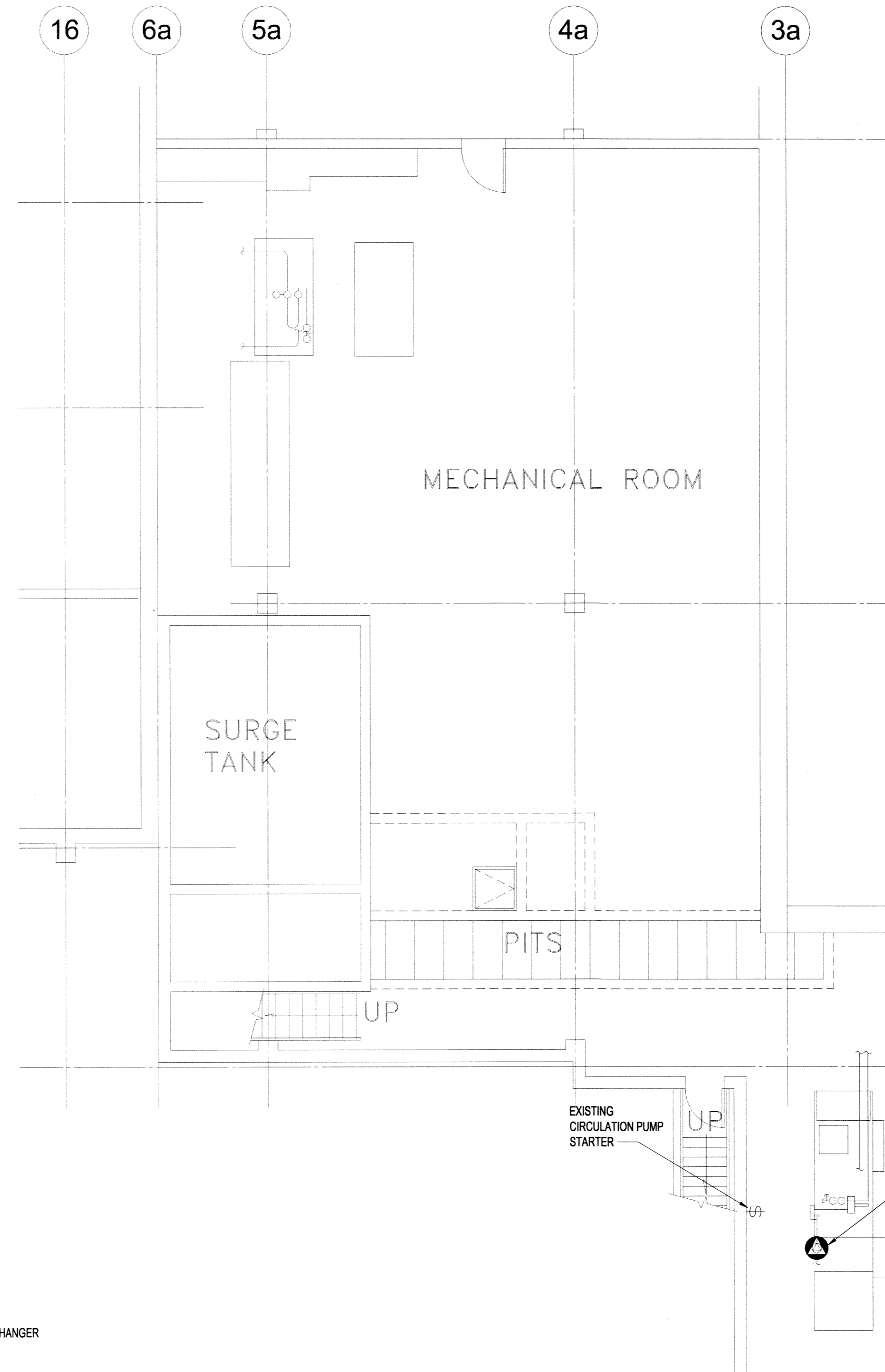
ELECTRICAL ROOM PLAN - NEW SCALE: 1:75
