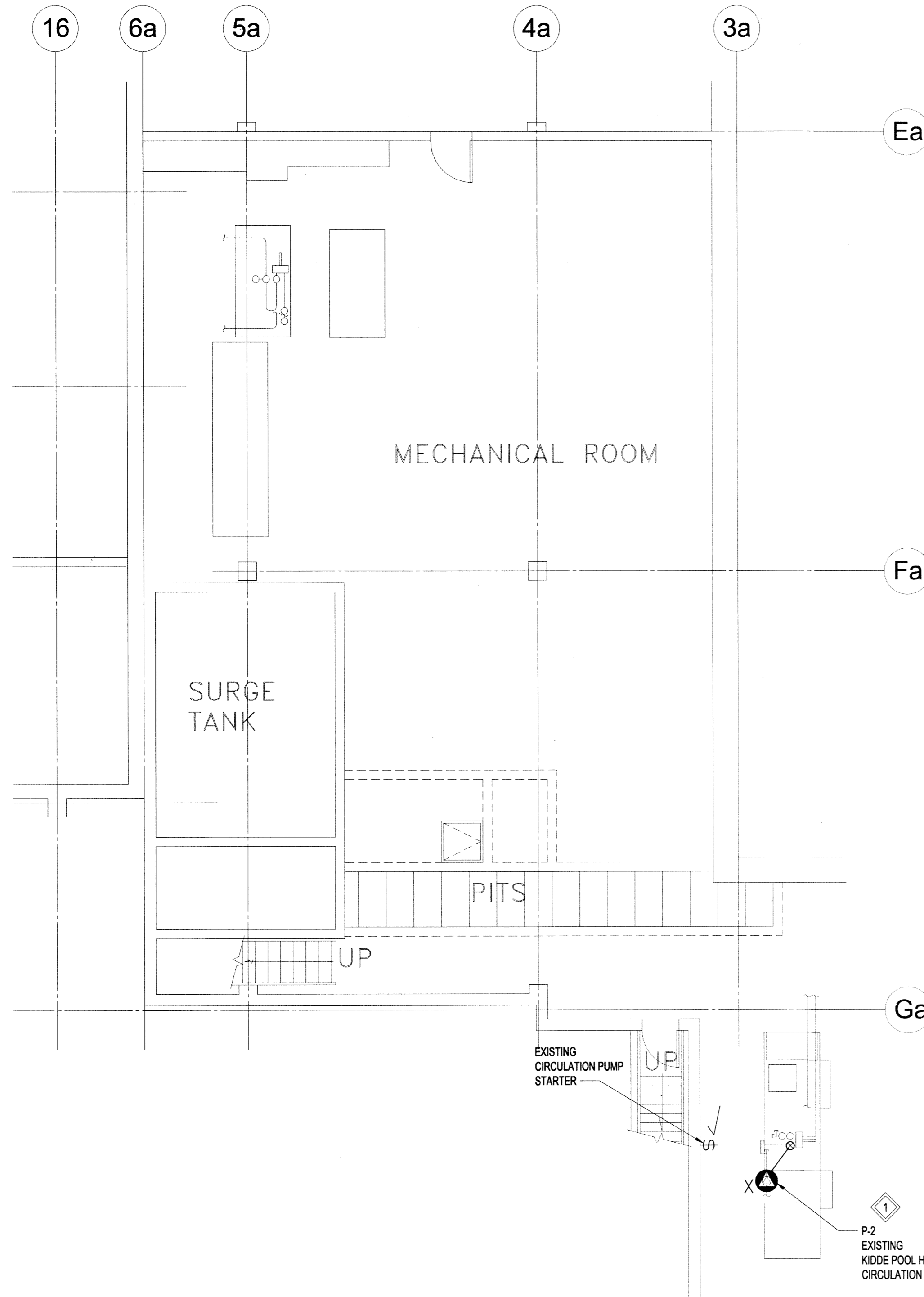
ELECTRICAL ROOM PLAN - DEMOLITION SCALE: 1:75
