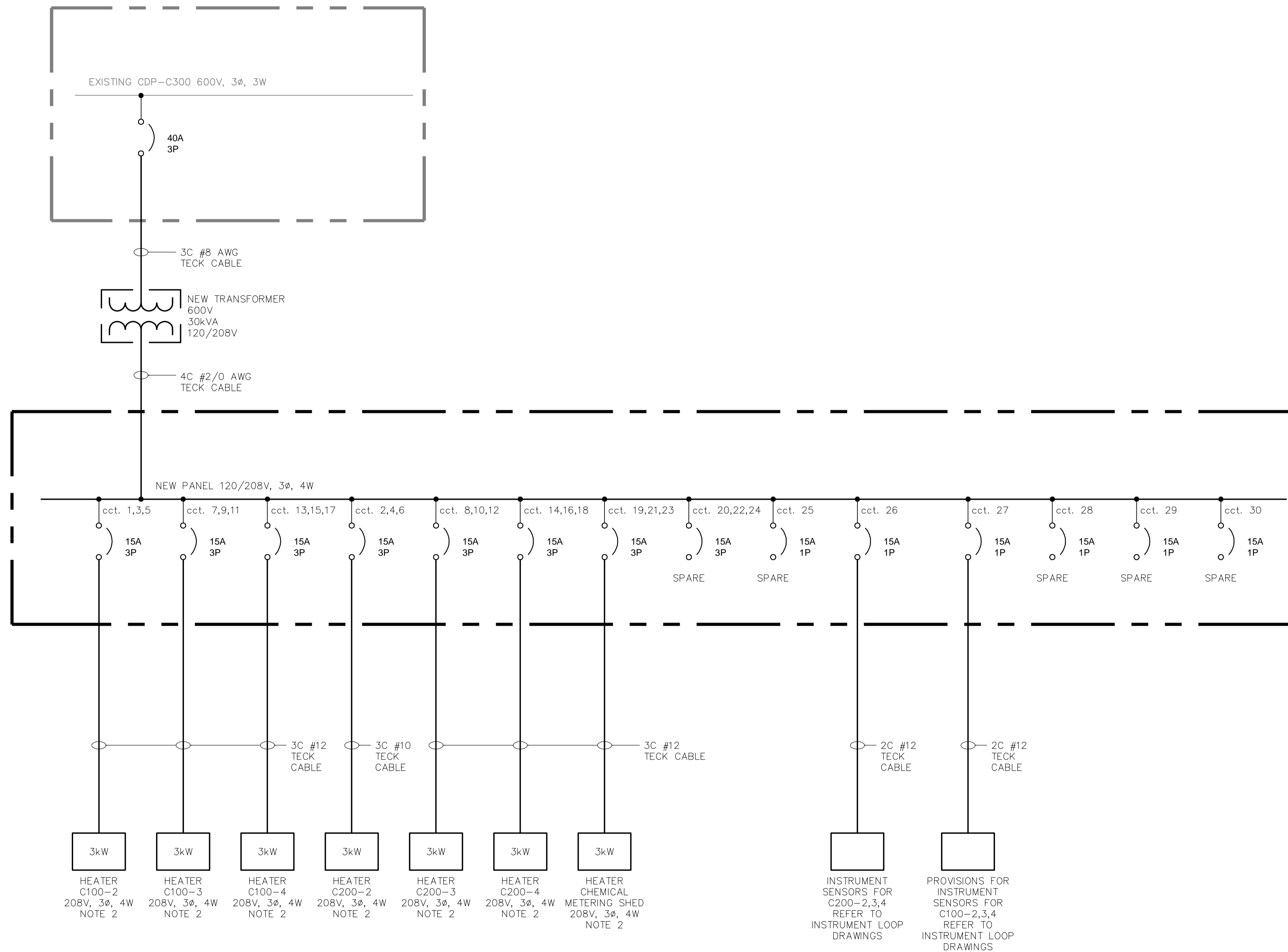
SINGLE LINE DIAGRAM SCALE : N.T.S.
