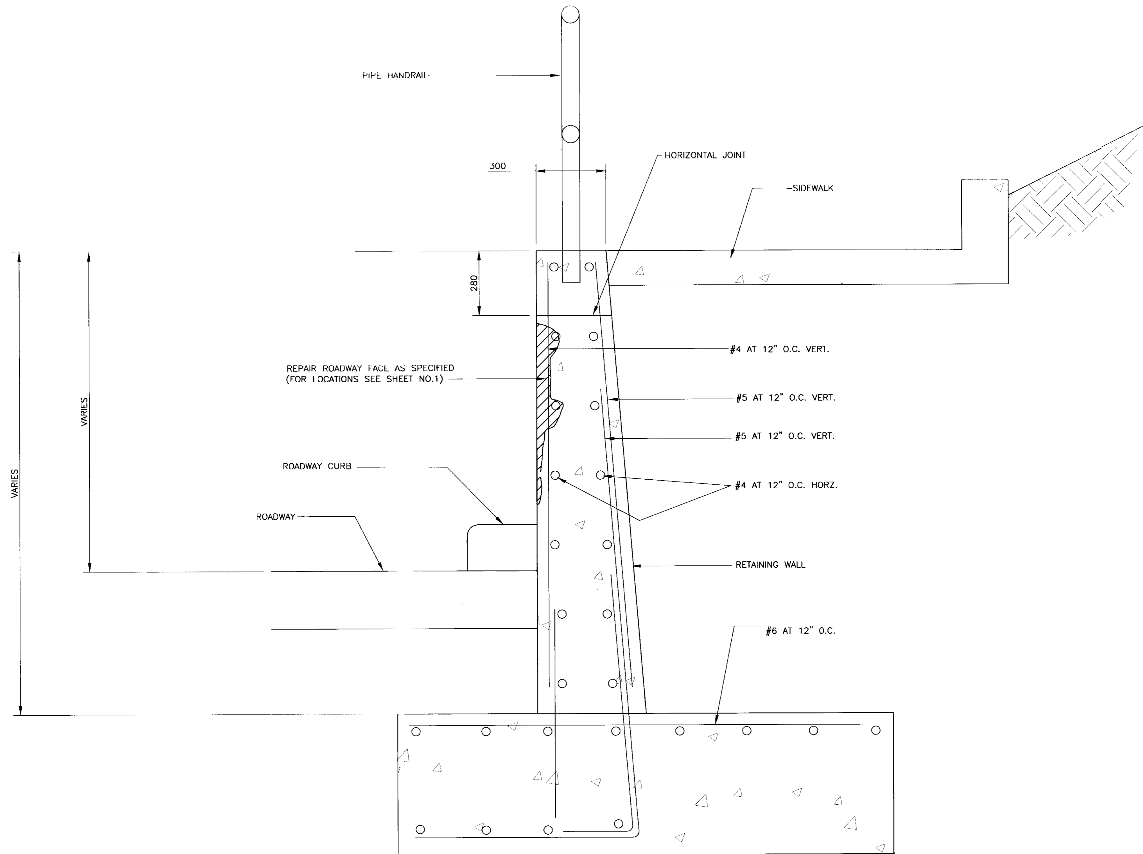
TYPICAL EXISTING RETAINING WALL SECTION 1: 10
