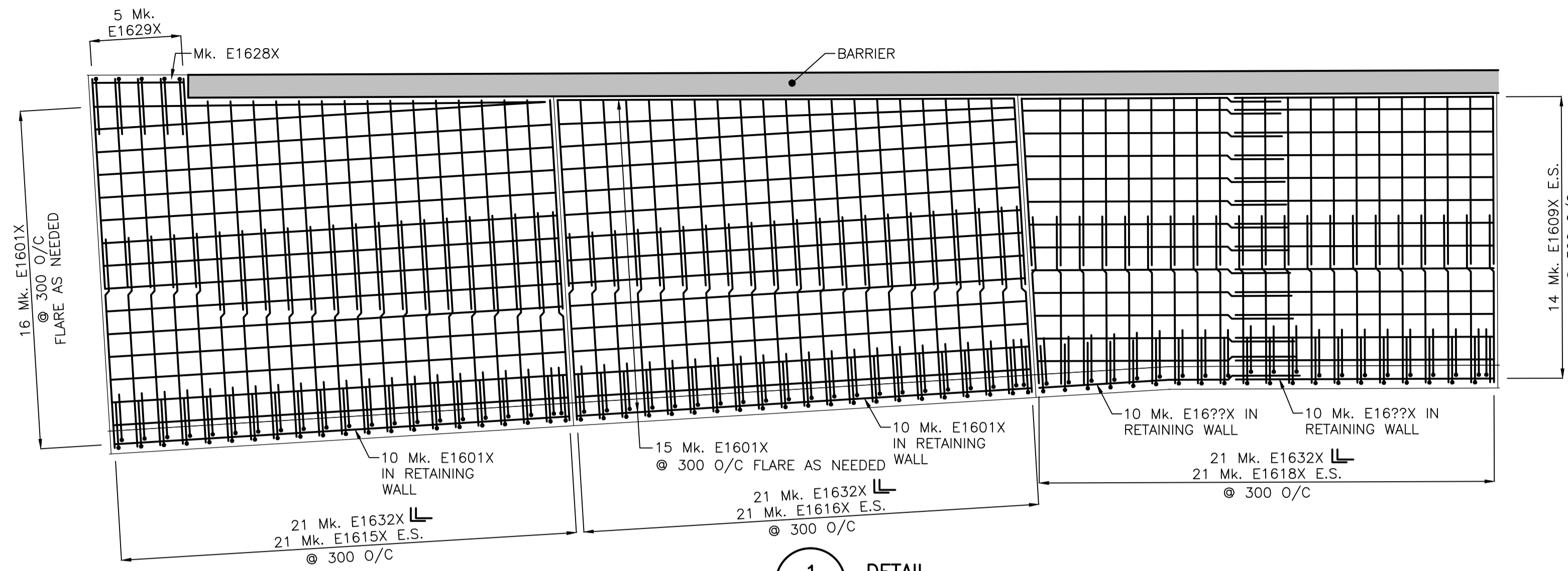
1 DETAIL 46 47 1:50
