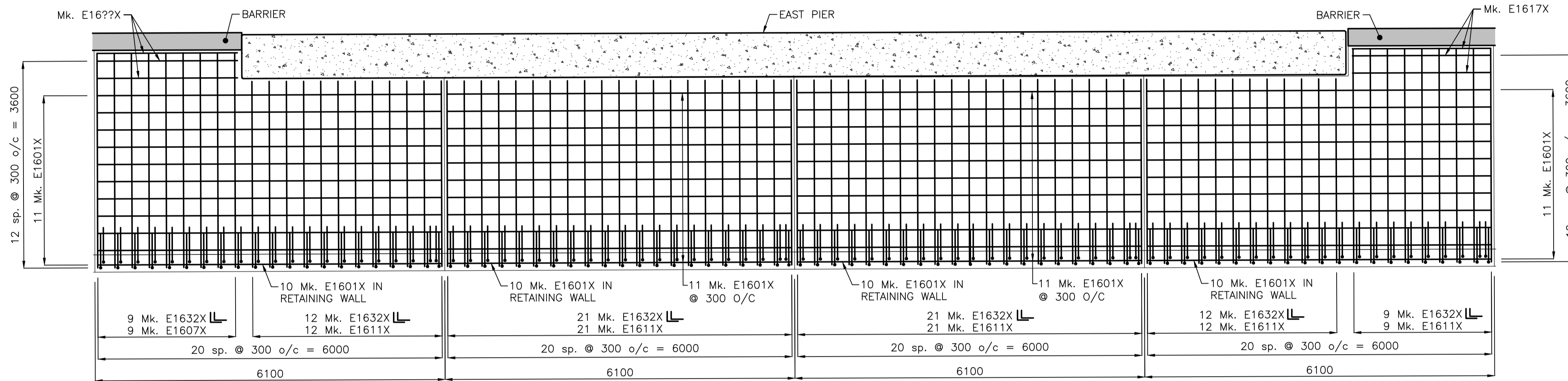
4 DETAIL 46 47 1:50
