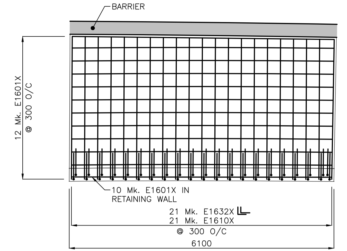
3 DETAIL - TYPE E TYP. OF 7 46 47 1:50
