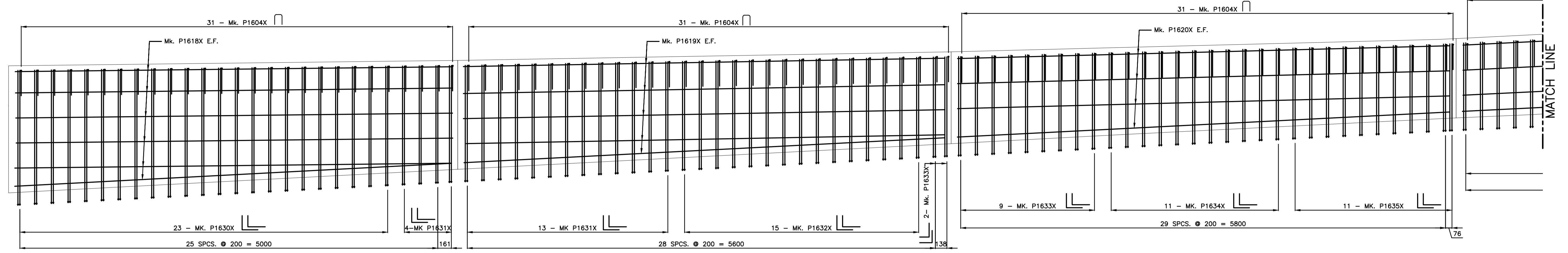
NORTH EAST PARAPET WALL REINFORCING 1:25
