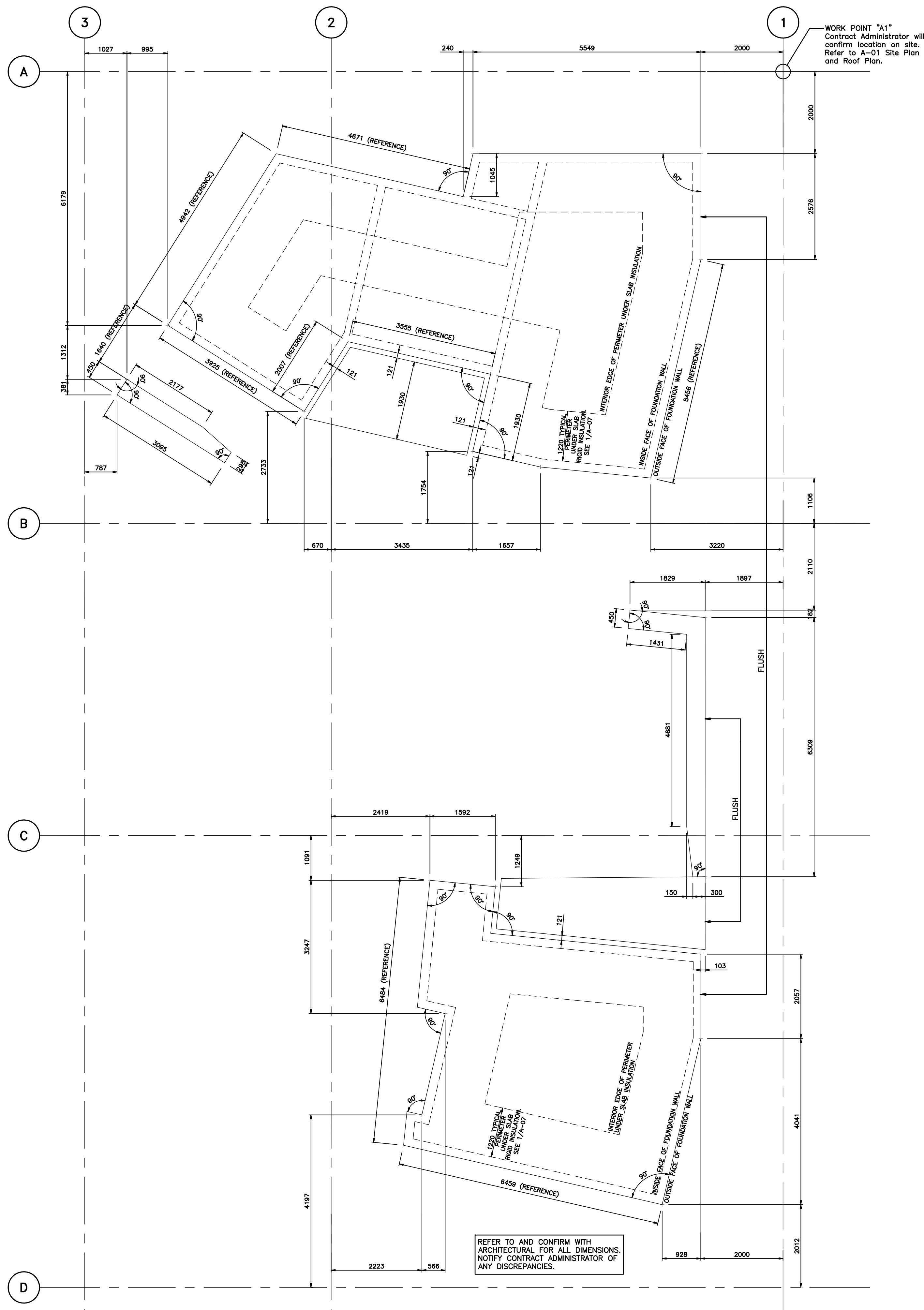
FOUNDATION LAYOUT PLAN 1 : 60
