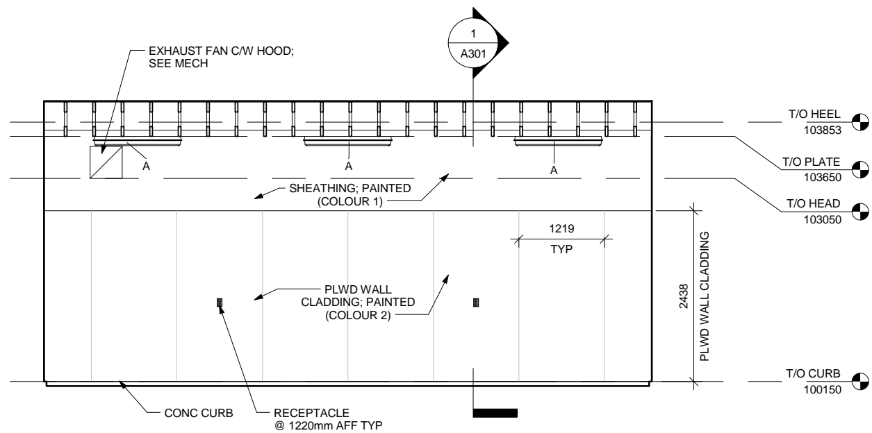
1 NORTH INTERIOR ELEVATION 1:75
