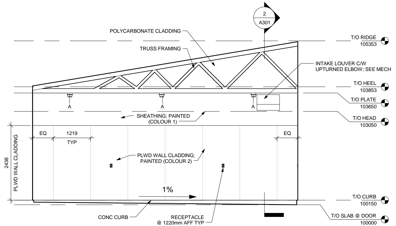
2 EAST INTERIOR ELEVATION 1:75
