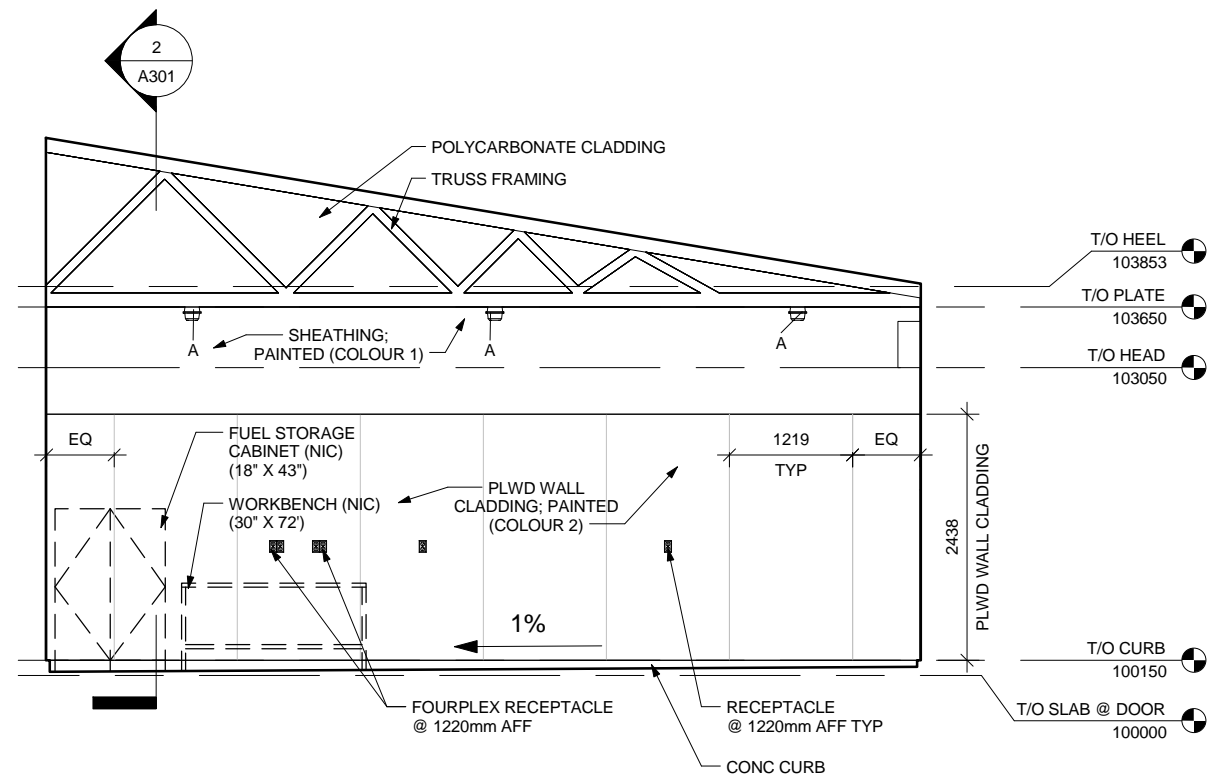
4 WEST INTERIOR ELEVATION 1:75
