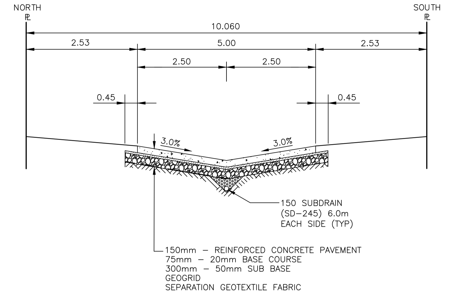
TYPICAL CROSS SECTION N.T.S
