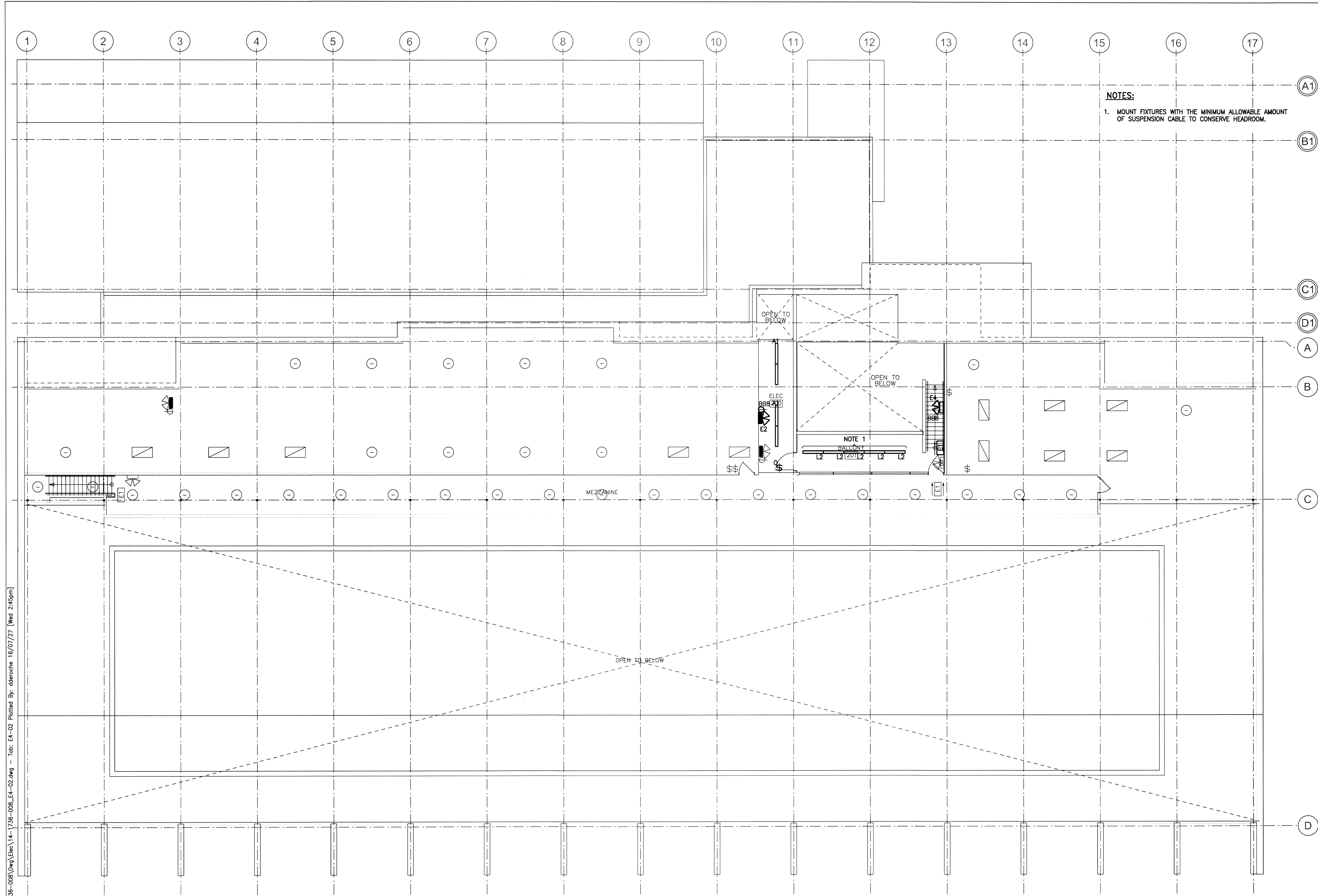
1 MEZZANINE LIGHTING PLAN - NEW 2000 0 2000 4000 6000 8000 SCALE: 1:100mm (24"x36")
