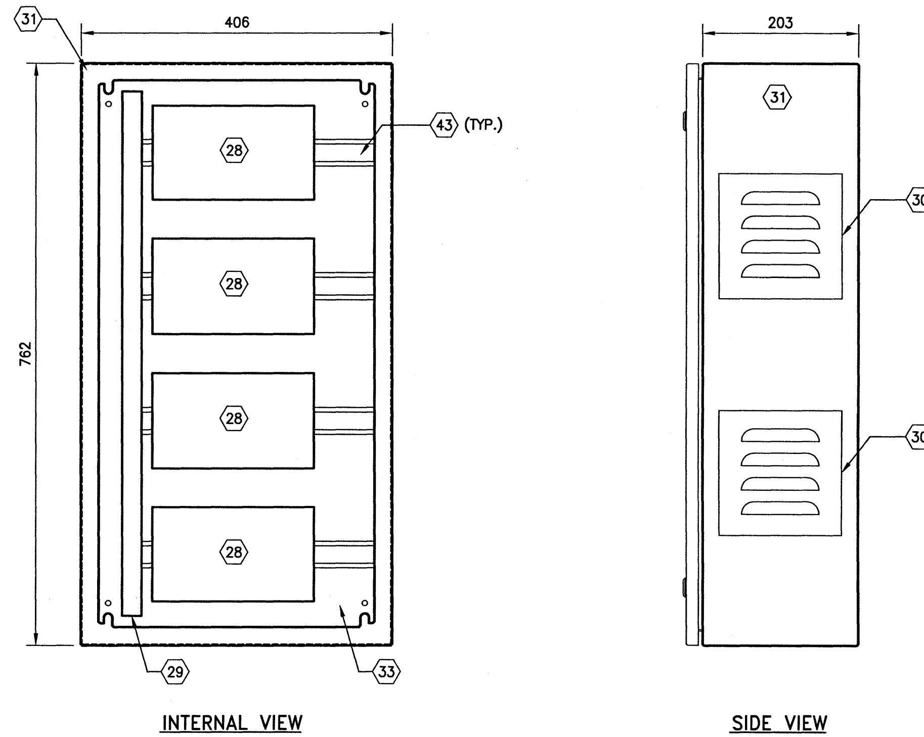
1 PSP-Z800 BATTERY ENCLOSURE 100 0 100 200 300 400 SCALE: 1:5mm (A1)
