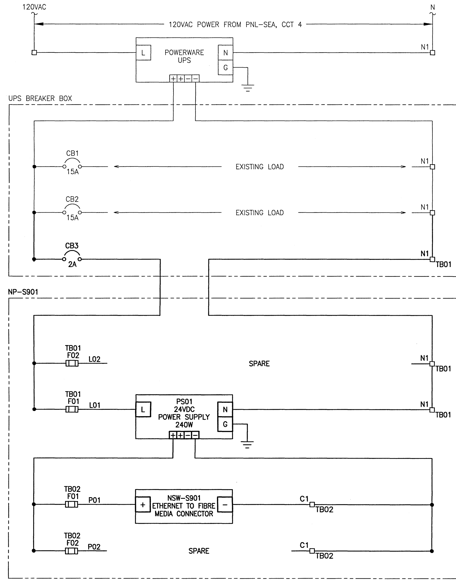
1 NP-S901 AND UPS BREAKER BOX SCHEMATIC DIAGRAM SCALE: N.T.S.
