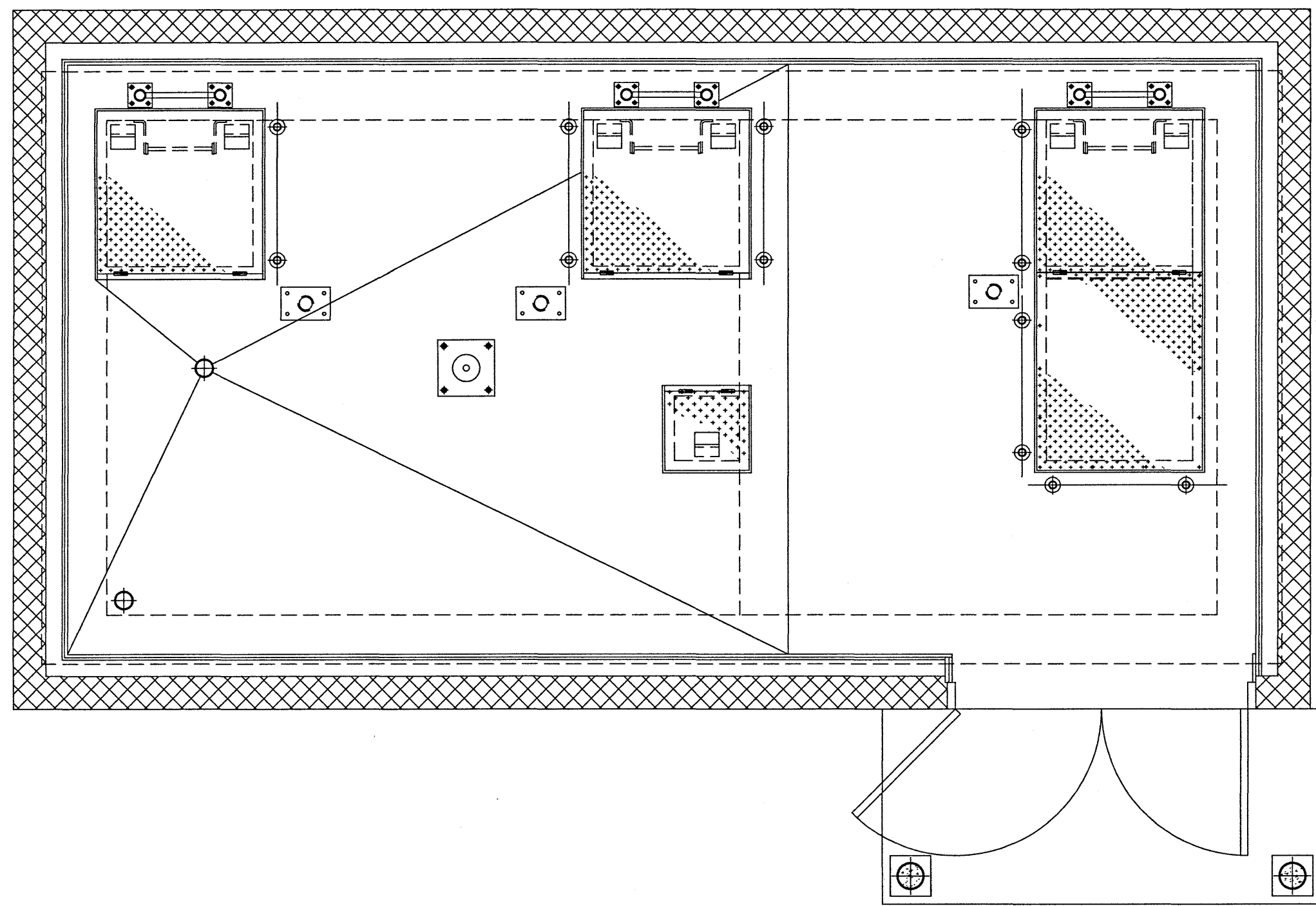
AREA CLASSIFICATION - MAIN FLOOR
