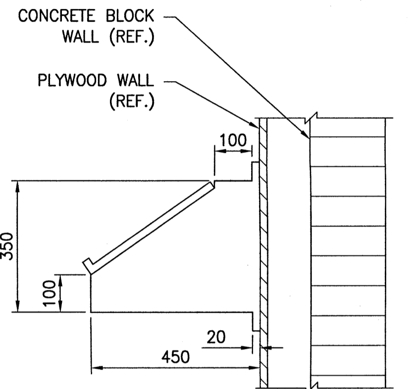
4 WALL MOUNTED CABINET SECTION SCALE: 1:10mm METRIC (A1)
