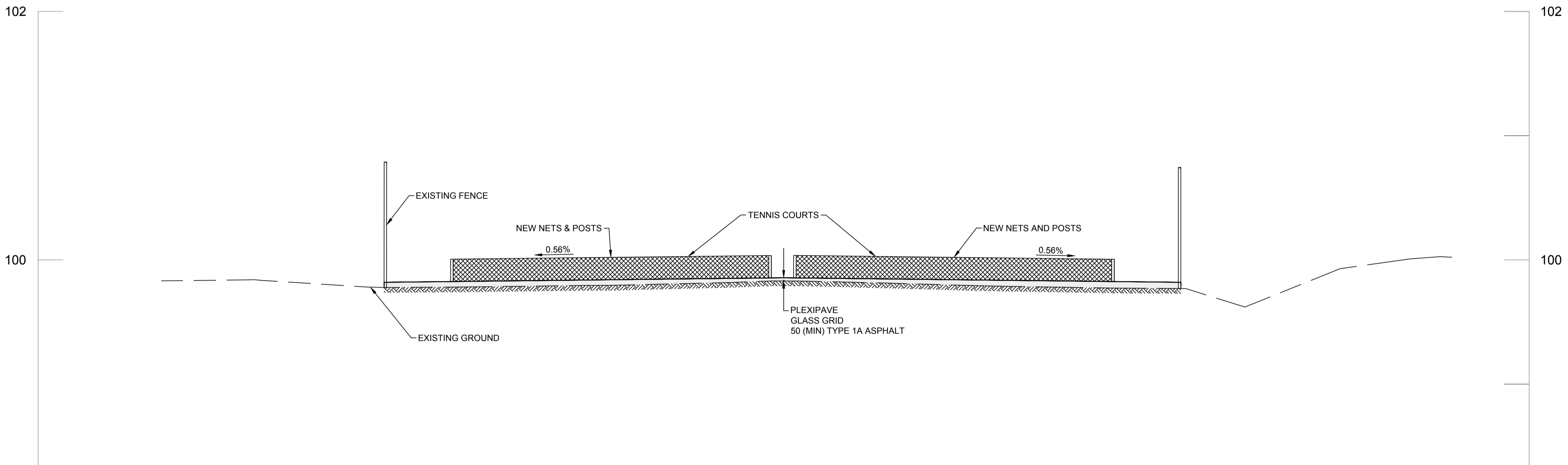
B PAVEMENT STRUCTURE - LINDEN WOODS TENNIS COURT Scale: H 1:100 V 1:50
