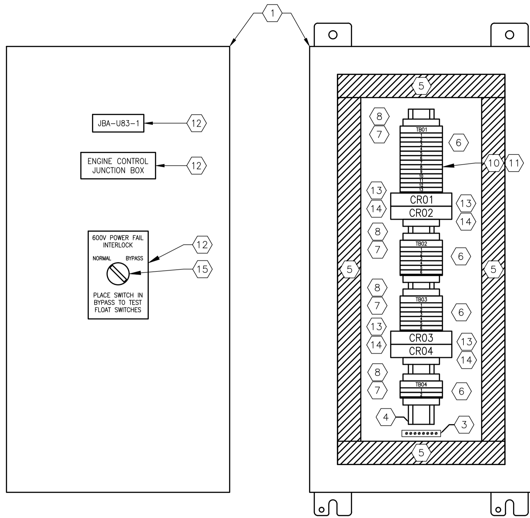
EXTERIOR PANEL VIEW SCALE: 1 : 3
