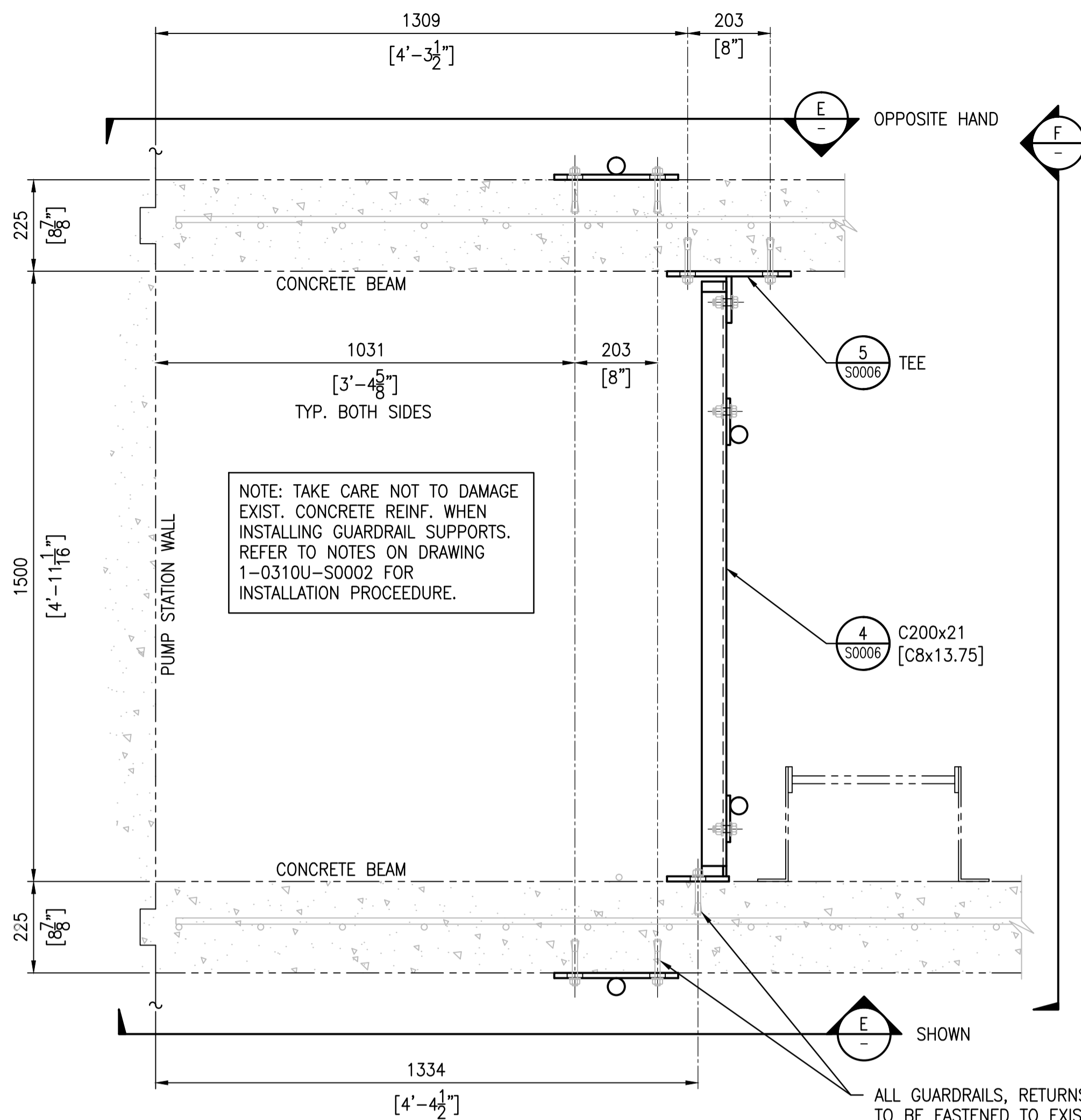
PLAN - ANCHOR BOLT LOCATIONS SCALE: 1 : 10
