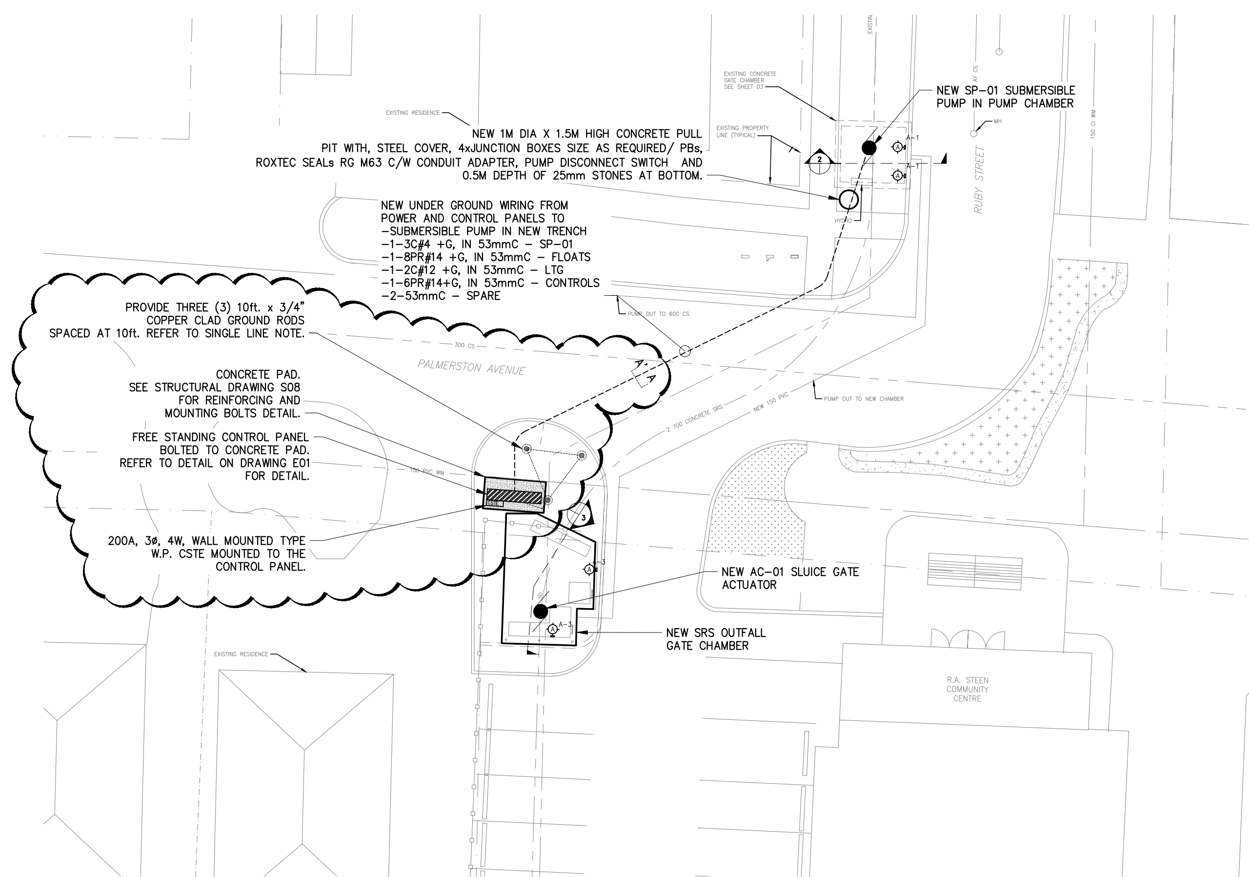
1 ELECTRICAL SITE PLAN SCALE: 1:200
