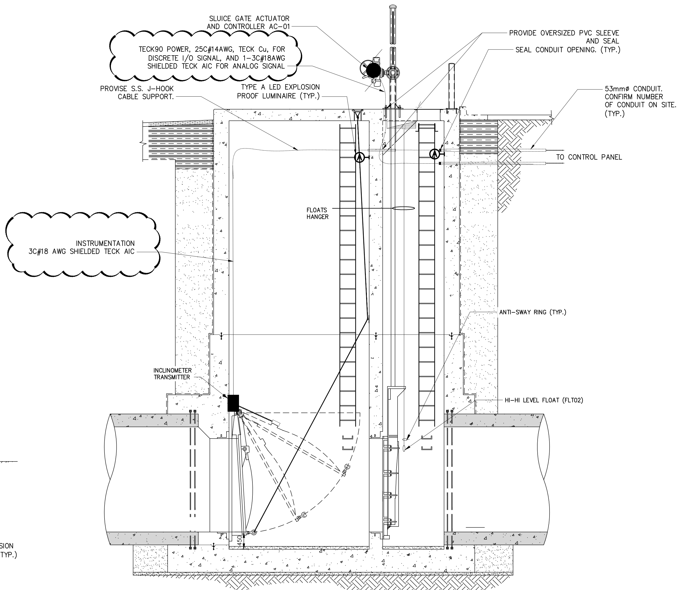
3 GATE CHAMBER SCALE: NTS
