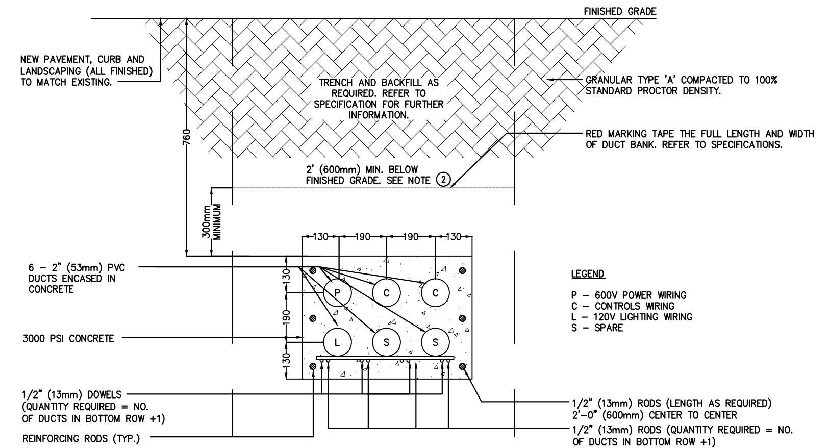
DUCTBANK DETAIL - SECTION 'A-A'
