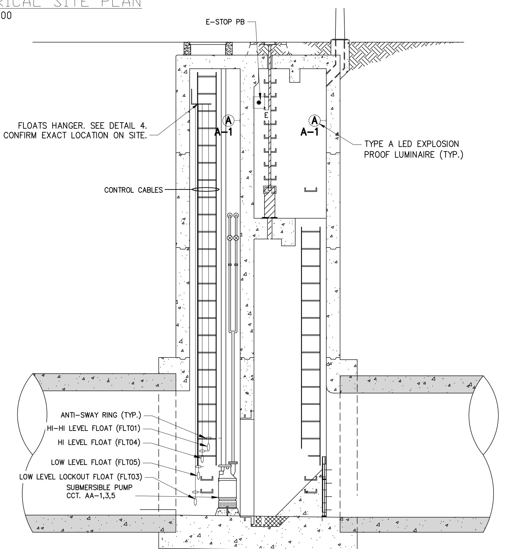
2 SUBMERSIBLE PUMP CHAMBER SCALE: NTS
