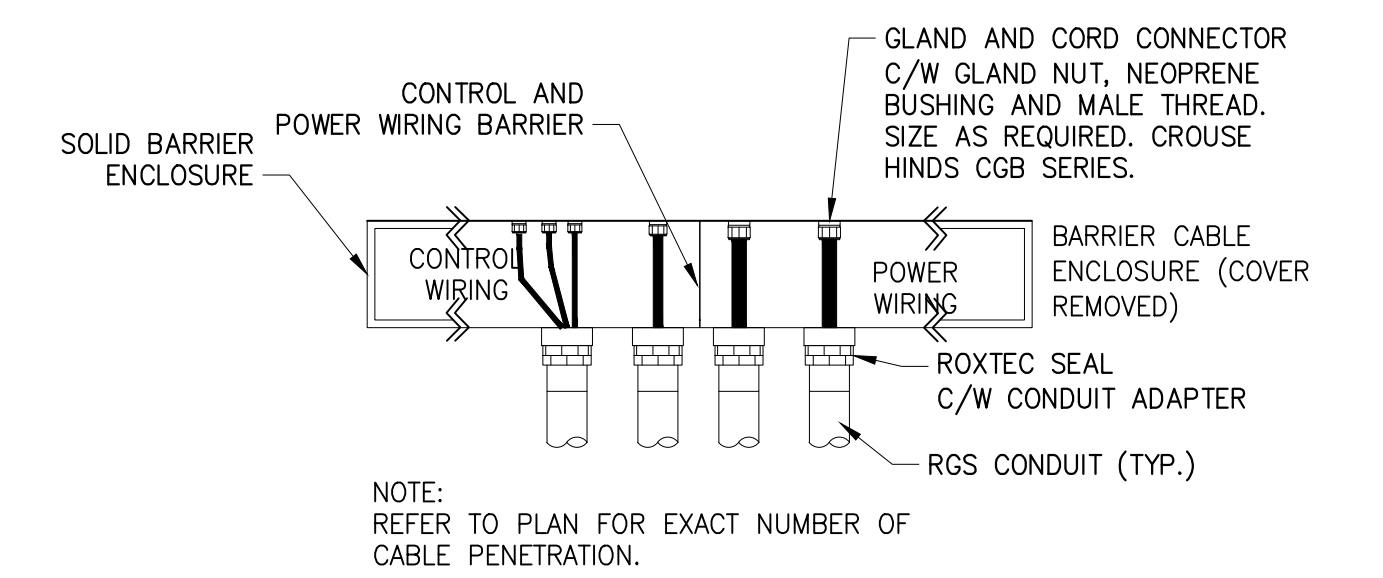
5 WIRING TO CONTROL PANEL (TYP.) SCALE: NTS
