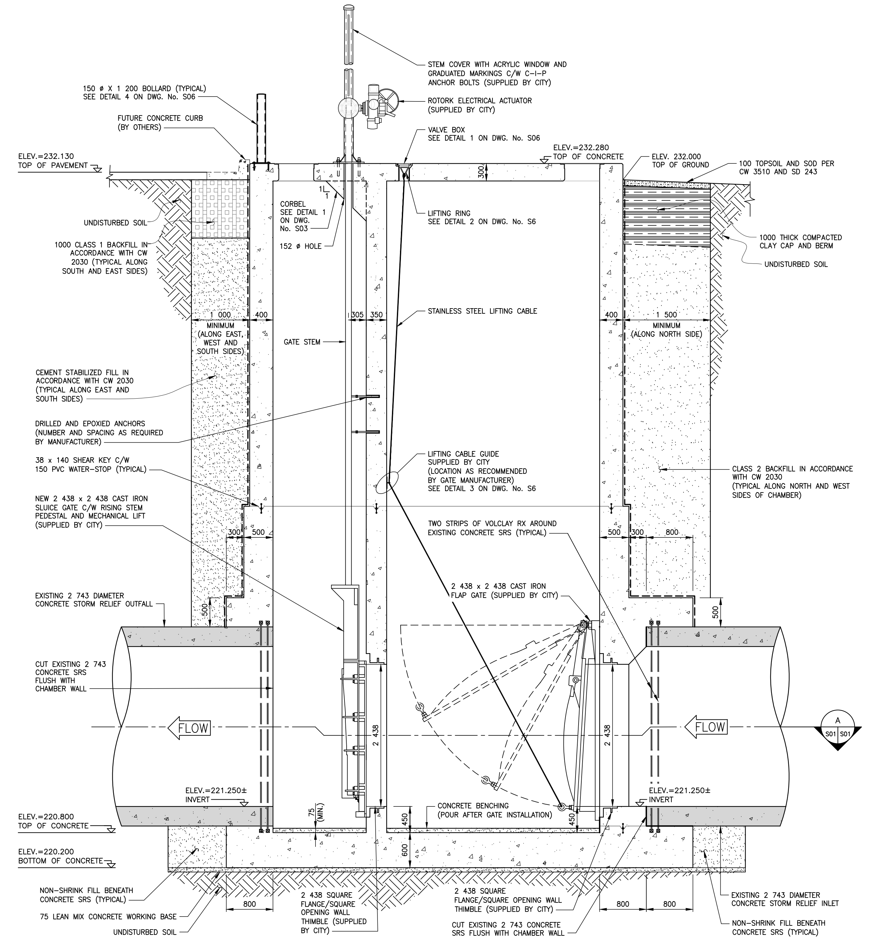
SECTION B
