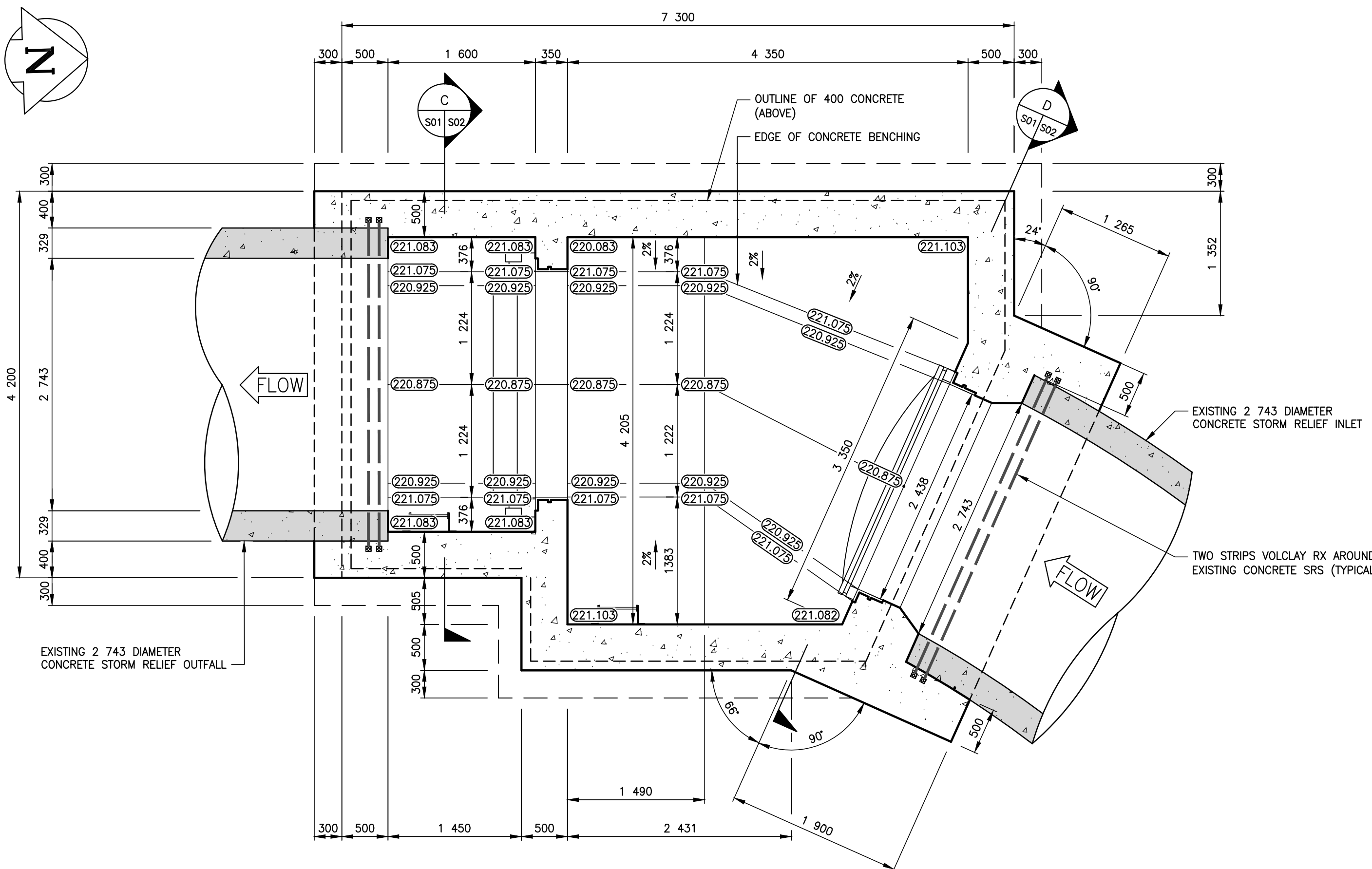
SECTION A
