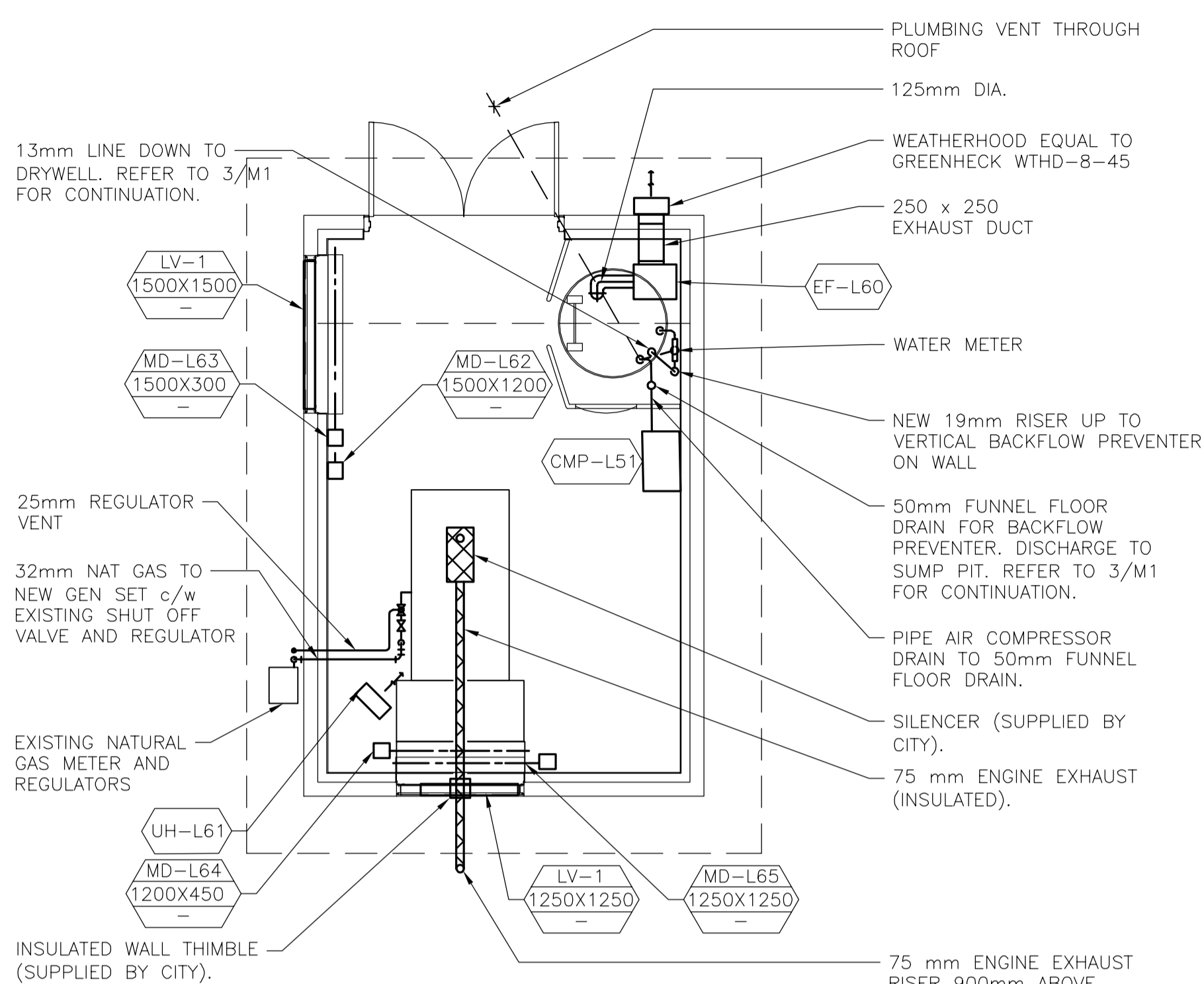
2 NEW WORK - BUILDING FLOOR PLAN M1 1:50
