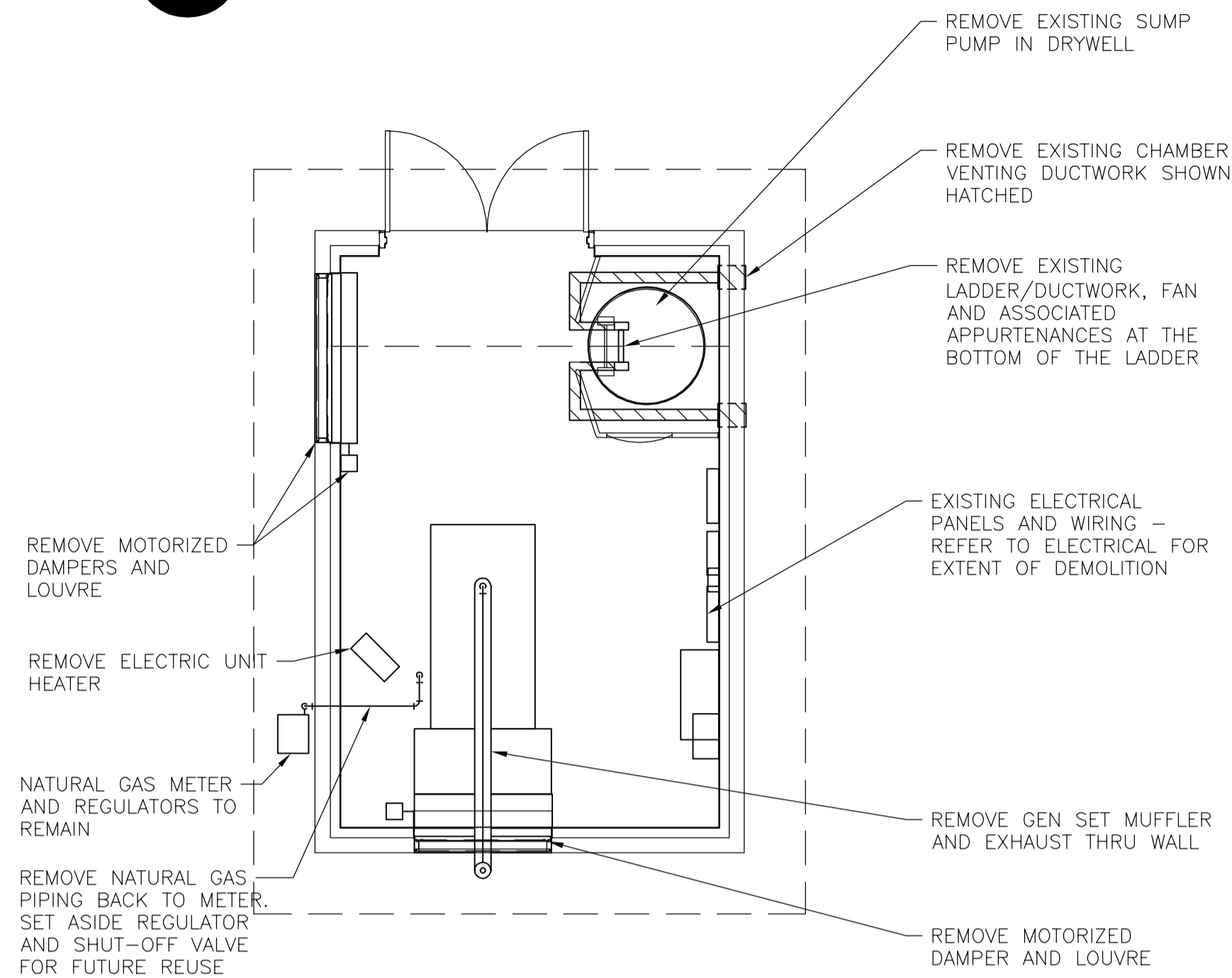
1 DEMOLITION - BUILDING FLOOR PLAN M1 1:50
