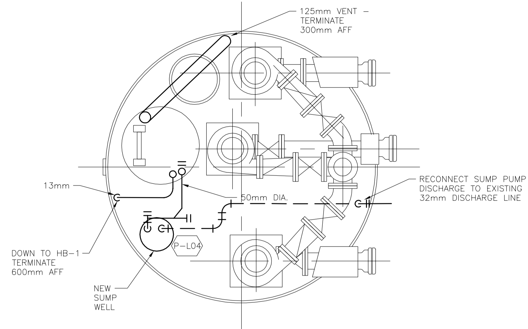
3 STATION FLOOR PLAN M1 1:25
