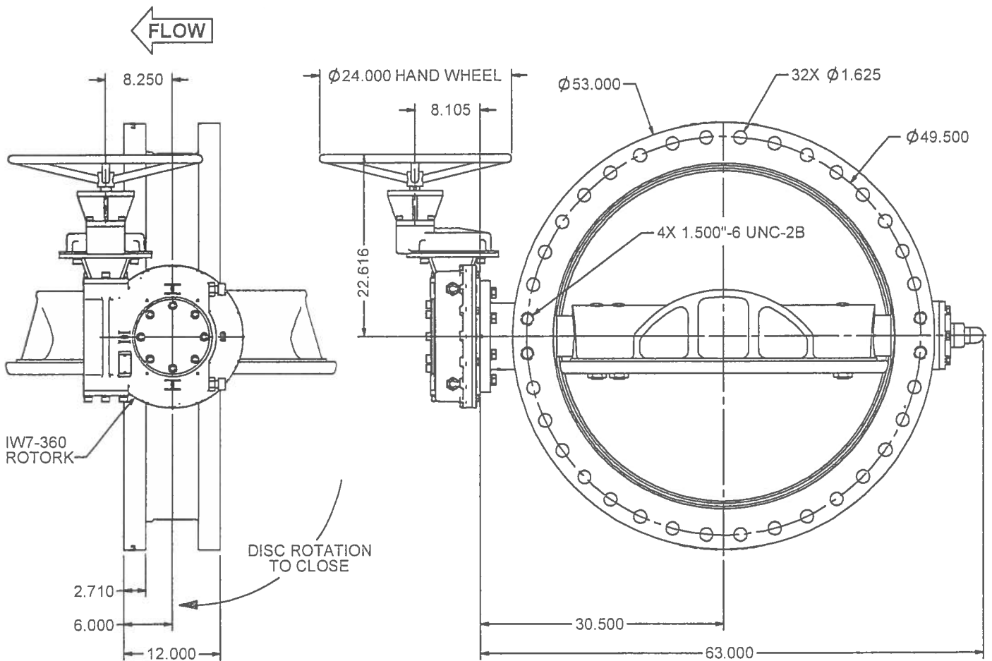
ASS'Y: "B1" (STD. MOUNTING)
