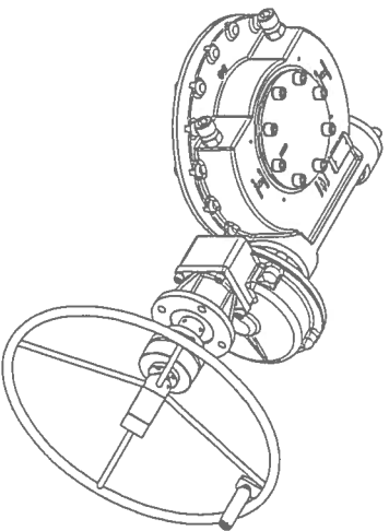
ISOMETRIC VIEW 1:1:1
