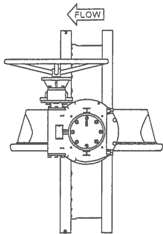
ASS'Y: "B1" (STD. MOUNTING)
