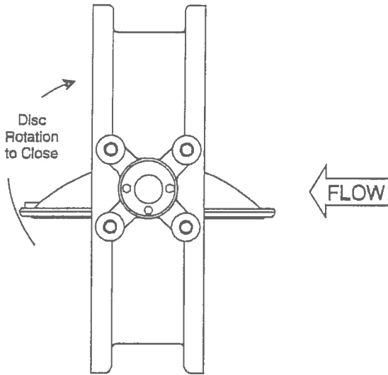
Figure 1--Flow Direction
