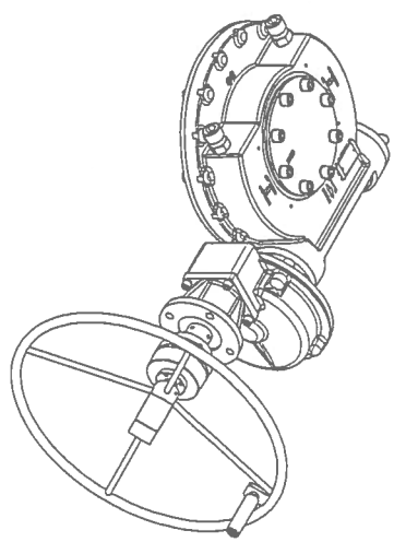
ISOMETRIC VIEW 1:11
