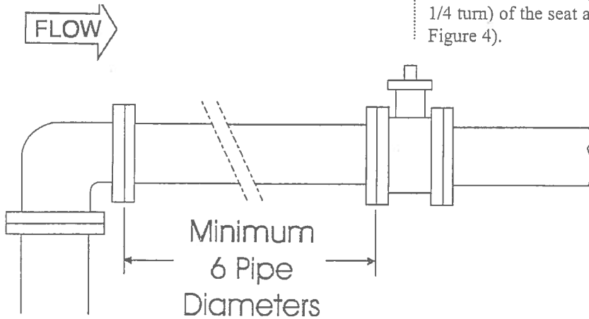
Figure 2--Valve Location
