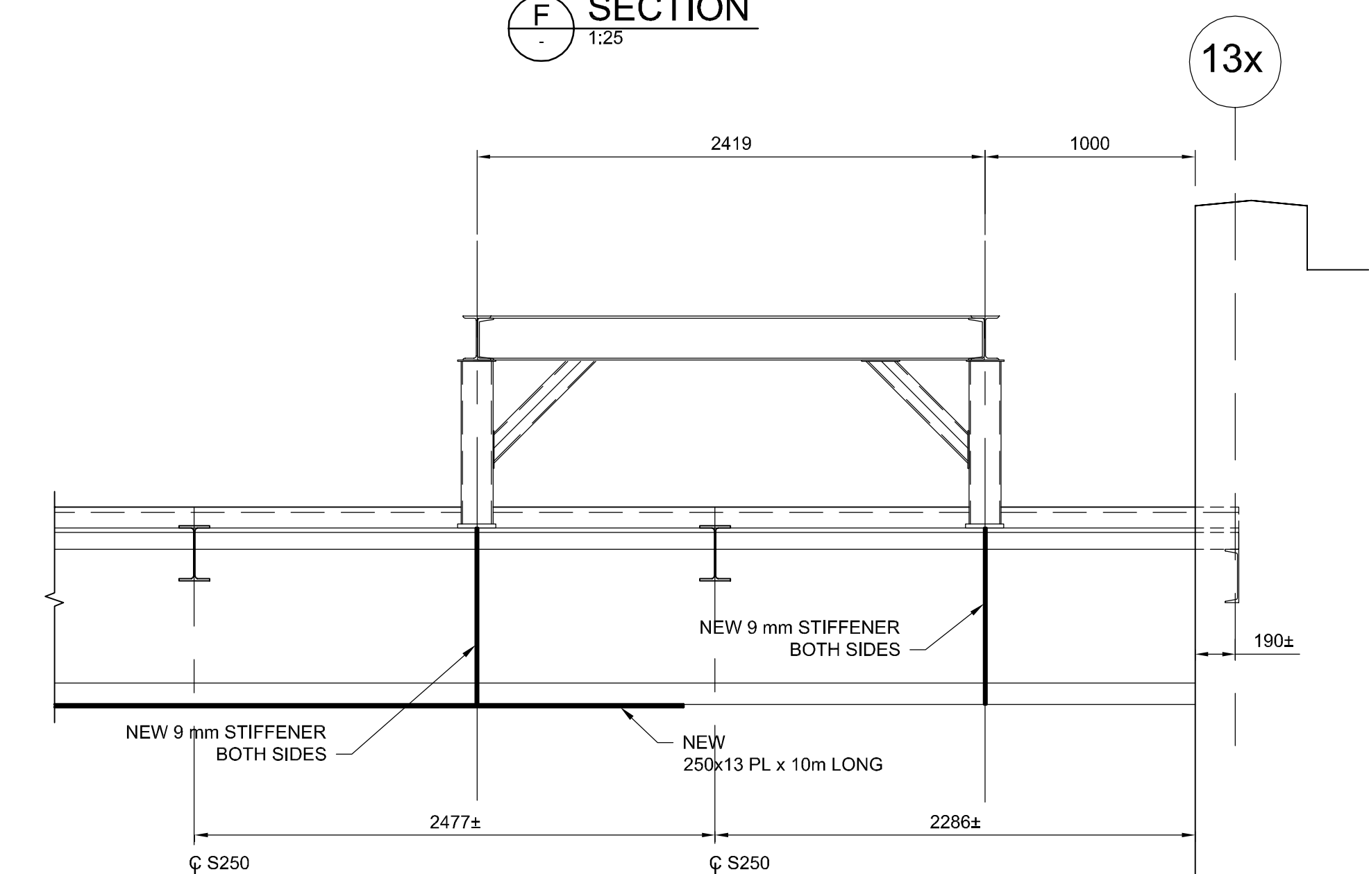
G SECTION 1:25
