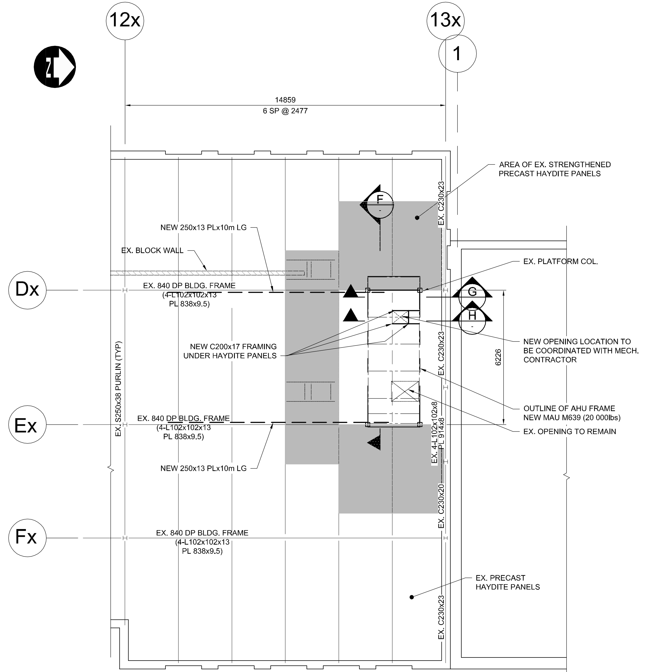
LAB BUILDING PARTIAL ROOF PLAN 1:100
