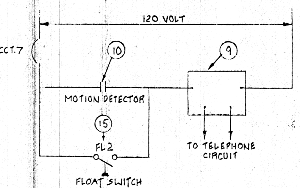
2 LOGIC DIAGRAM FOR ALARM PANEL CONNECTION 02
