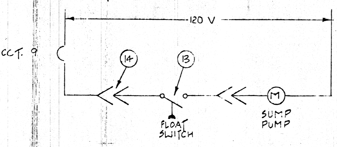
1 SUMP PUMP CONTROL SCHEMATIC 02 SEE DETAIL 3 02
