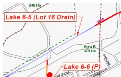
Site 8 Lot 16 Drain @ Plaza inlet* (Inlet Structure to 96" pipe)
