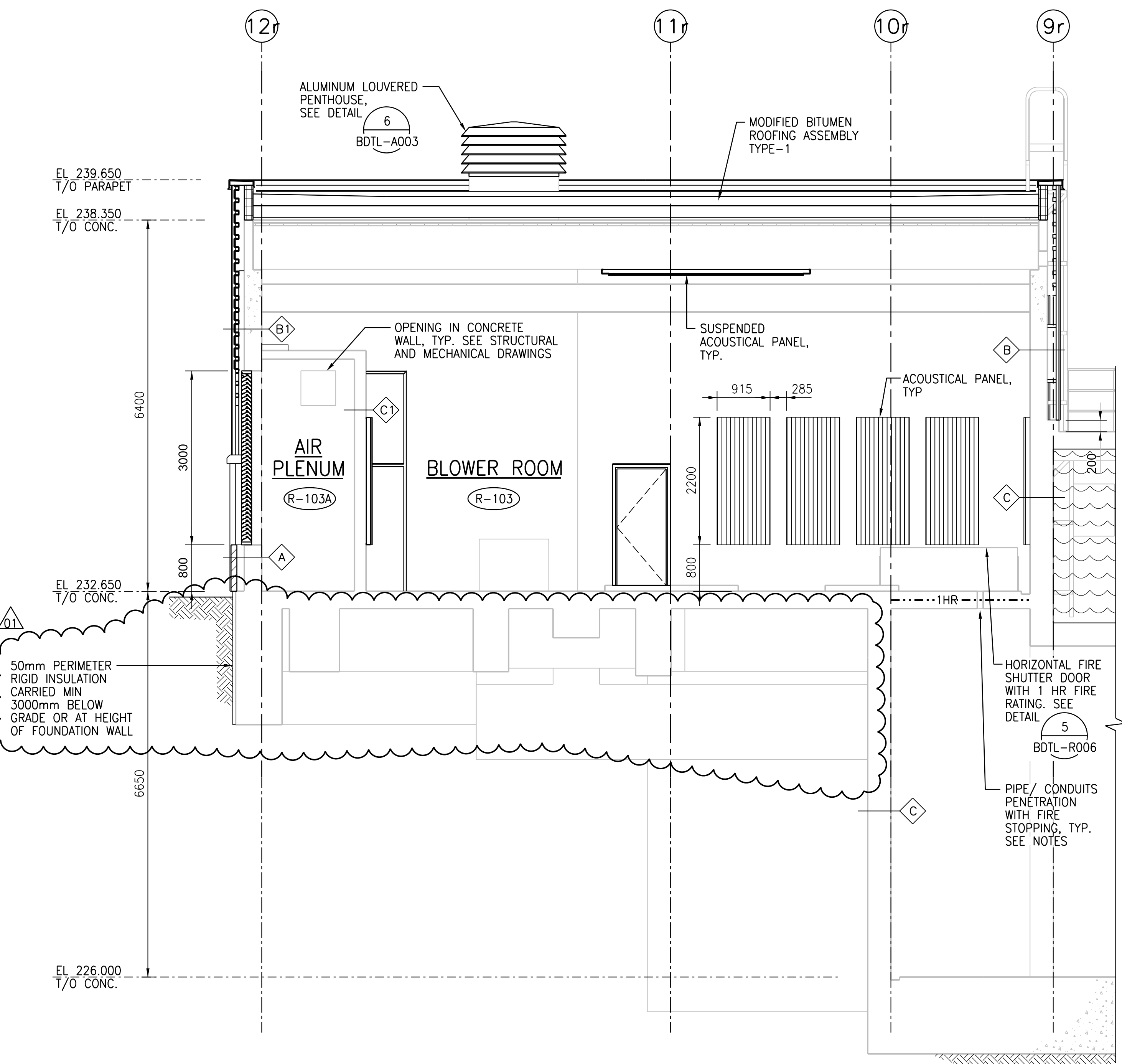
C SECTION C 1:50 BGAD-R003 BGAD-R004 BGAD-R005
