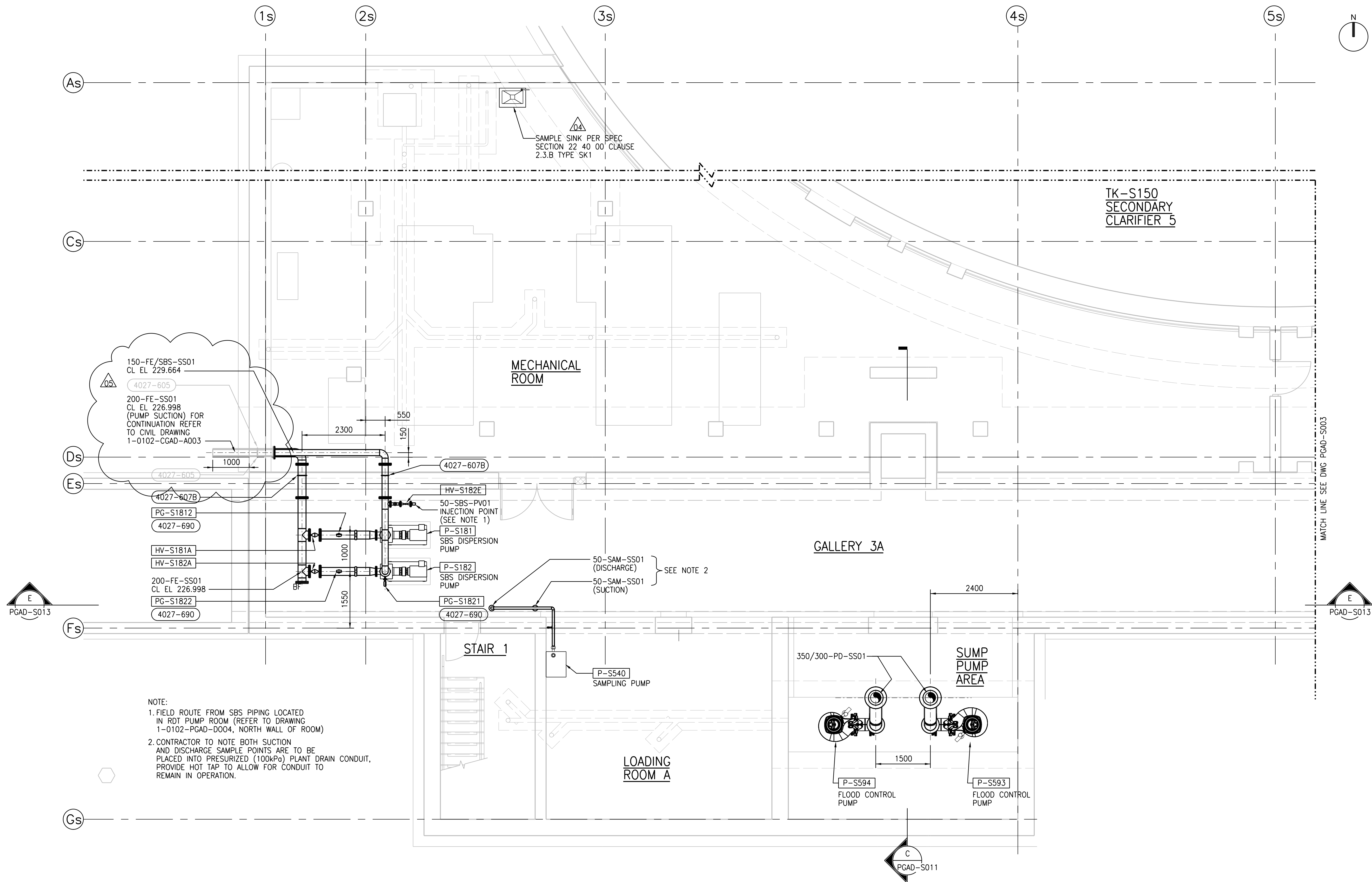
LOWER LEVEL PLAN - PART A 1:50
