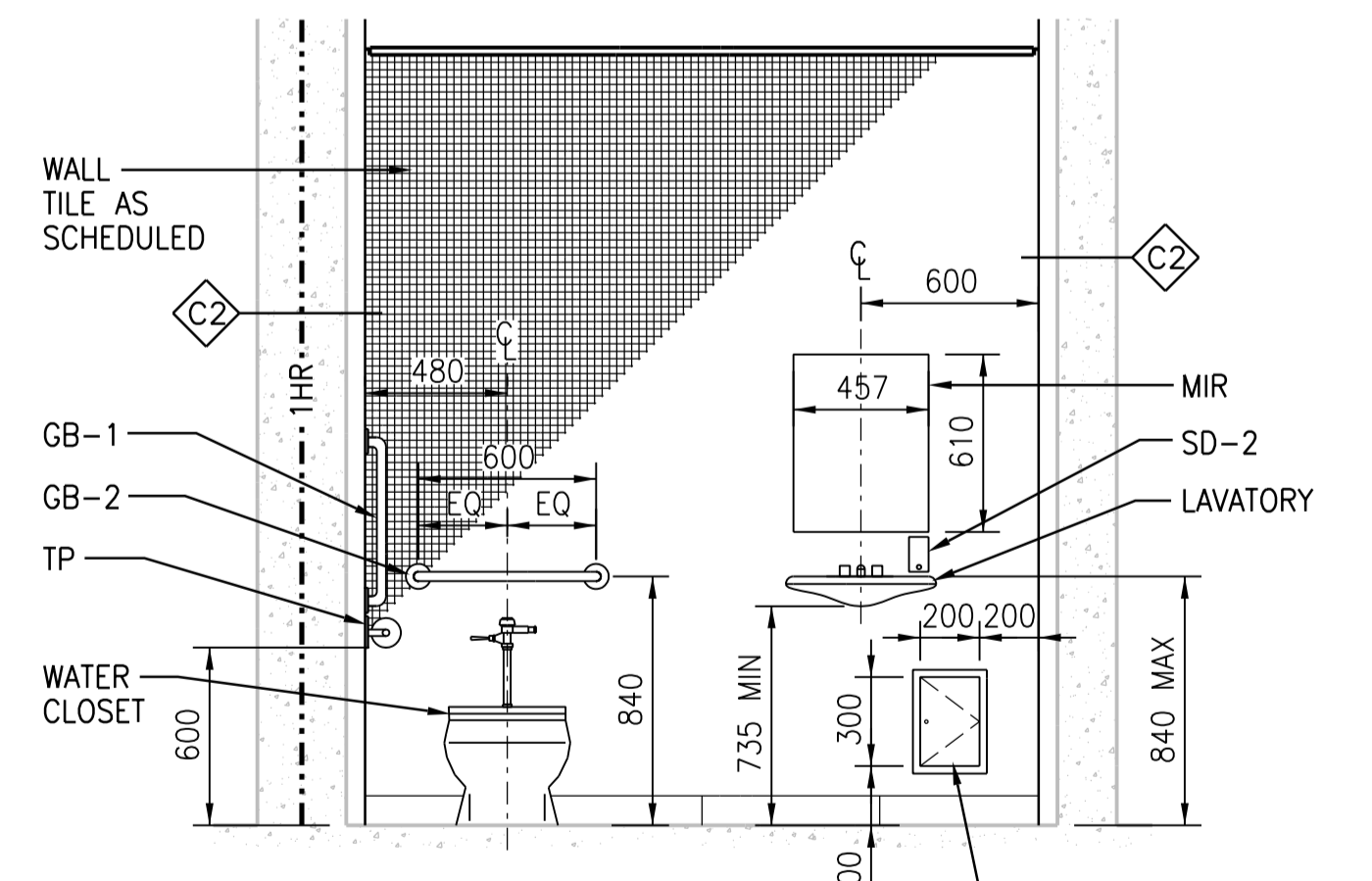
5 WASHROOM DETAILED SECTION 1:25
