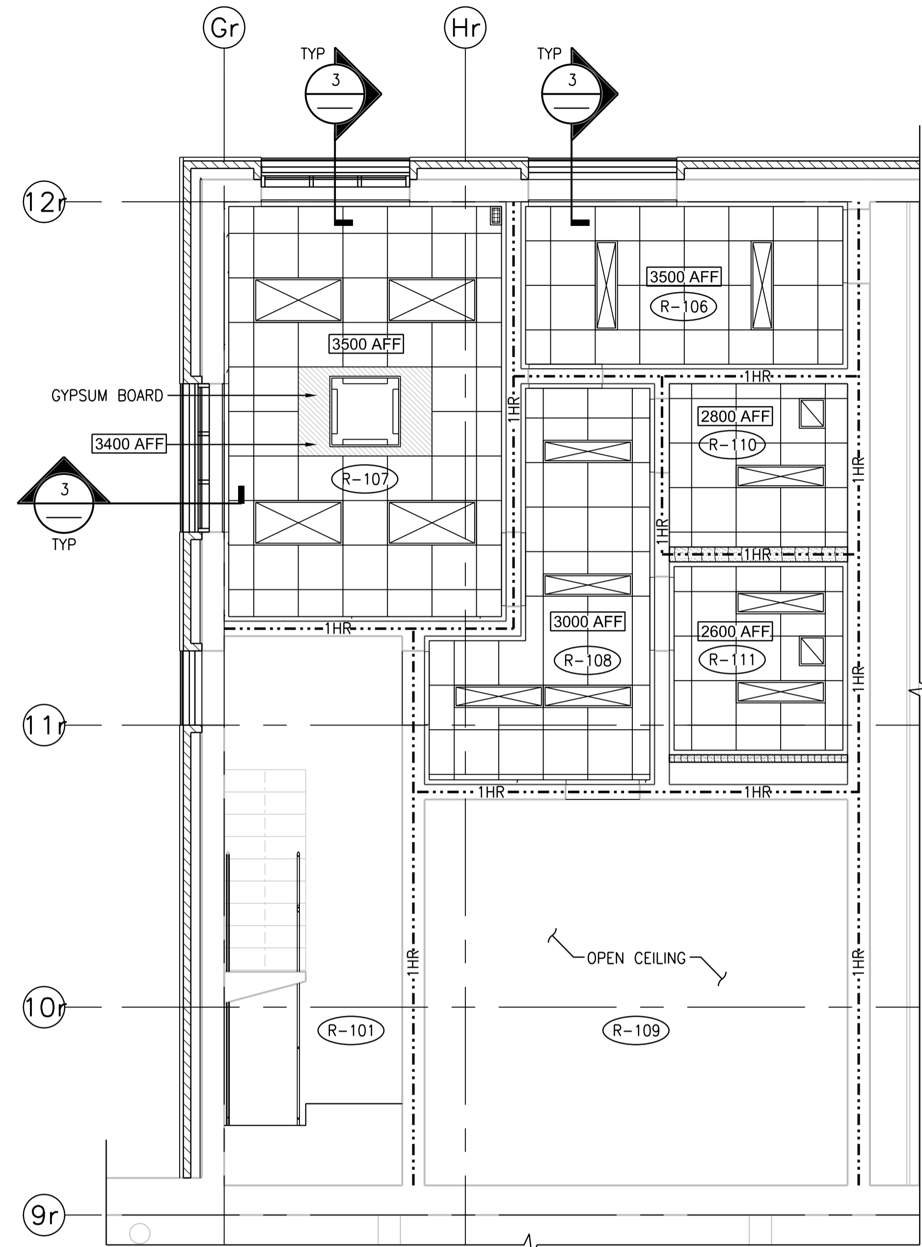
2 REFLECTED CEILING PLAN 1:50
