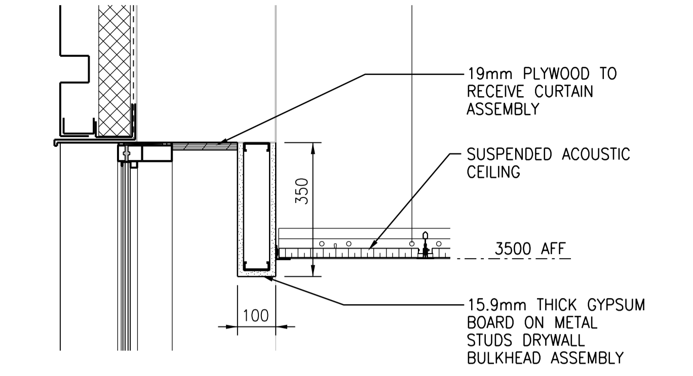
3 SECTION DETAIL NTS
