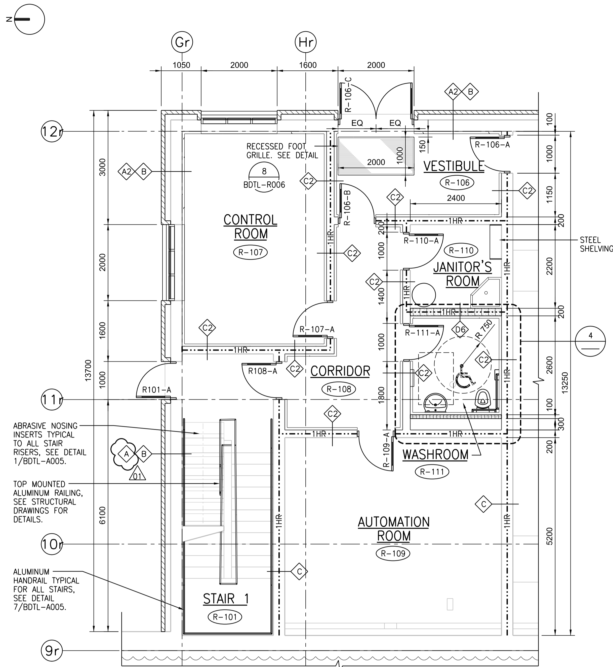
1 DETAILED PLAN 1:50 BCAD-R004
