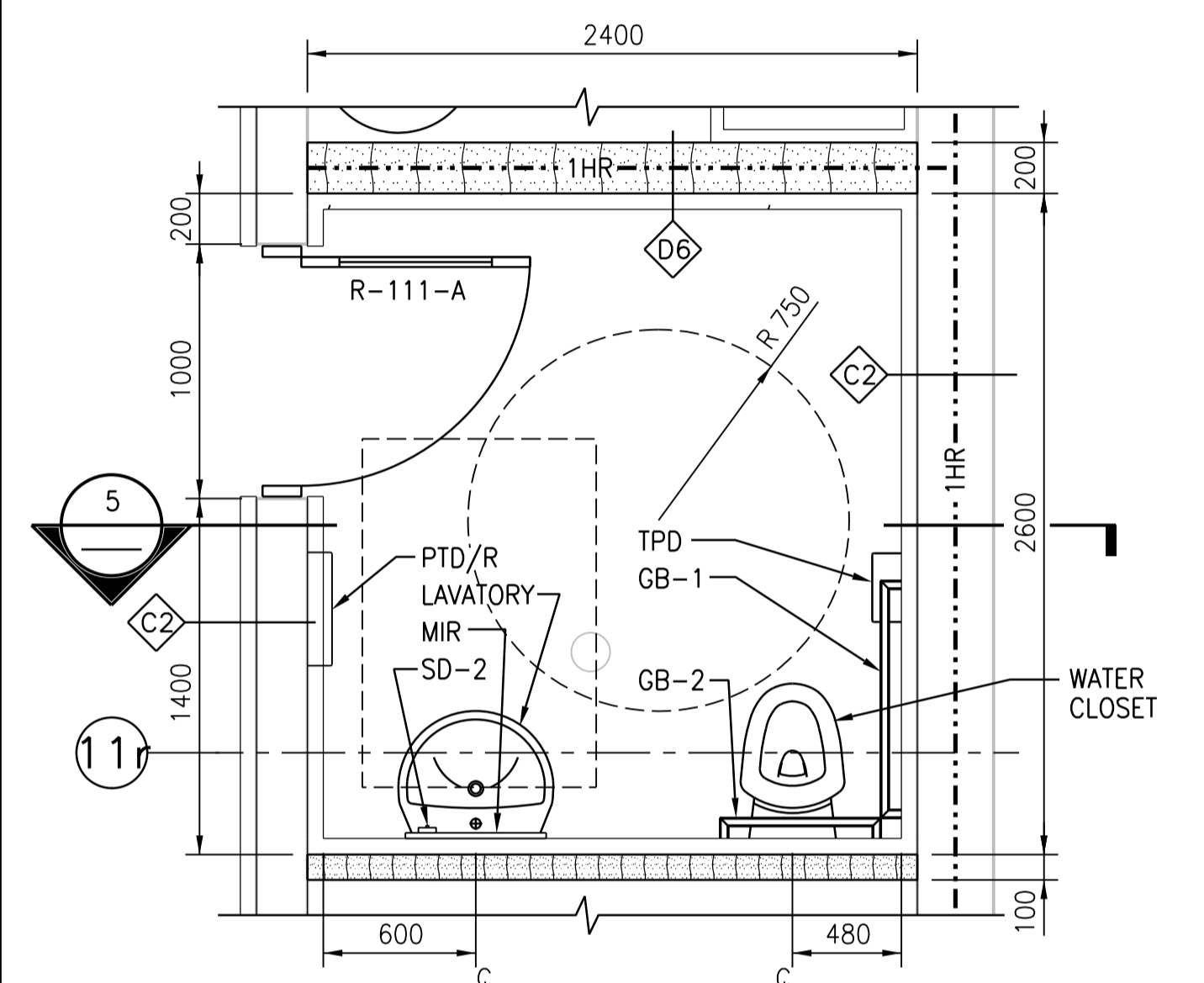
4 WASHROOM DETAILED PLAN 1:25 WASHROOM ACCESSORIES: MIR - MIRROR (457mm(W) X 914mm(H)) PTD/R - PAPER TOWEL DISPENSER AND RECEPTACLE SD-2 - WALL MOUNTED SOAP DISPENSER TP - TOILET PAPER DISPENSER GB-1 - GRAB BAR (915mm 45-DEGREES) GB-2 - GRAB BAR (610mm)
