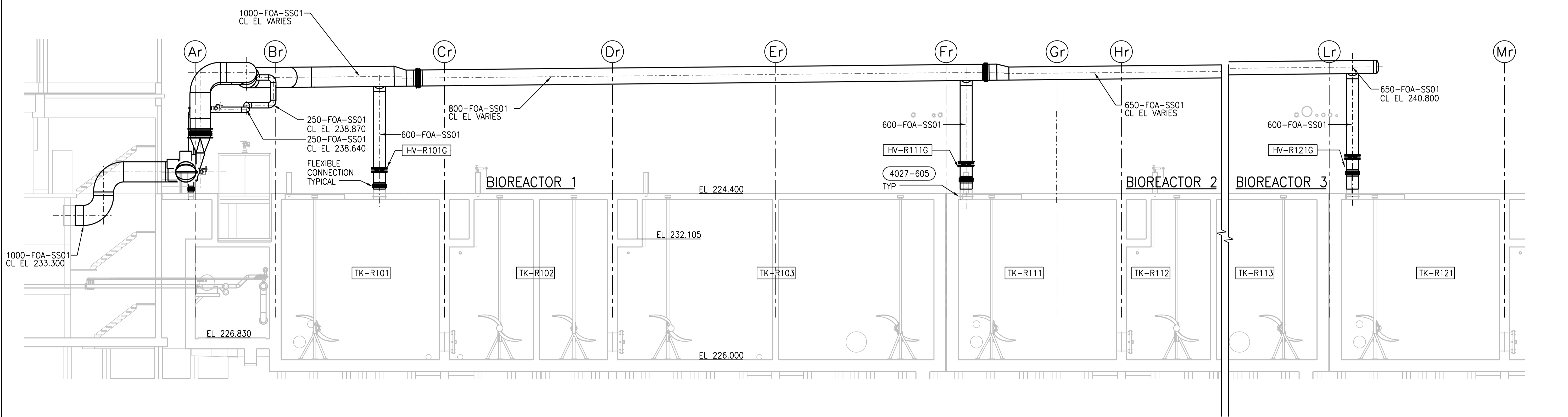
B SECTION 1:100 MGAD-R621
