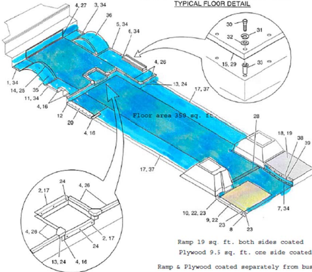
TYPICAL FLOOR DETAIL
