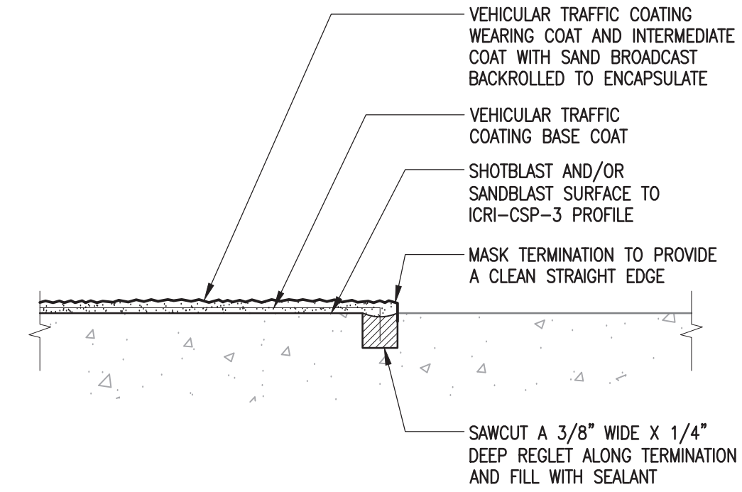
3 DETAIL AT HORIZONTAL TERMINATION - S6.1 N.T.S. (VEHICULAR TRAFFIC COATING)
