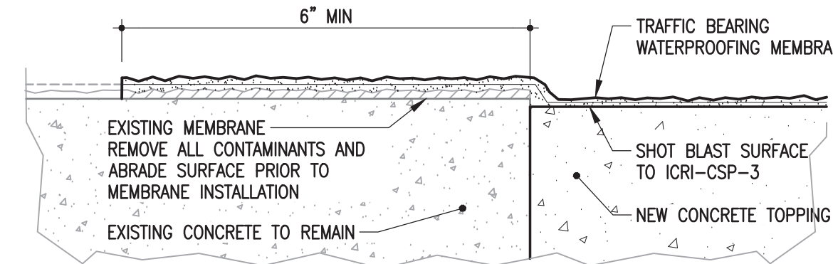
6 TYPICAL MEMBRANE REPAIR DETAIL - S6.1 N.T.S. (VEHICULAR TRAFFIC COATING)
