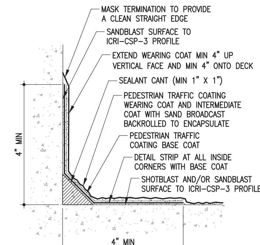
5 DETAIL AT INSIDE CORNER - S6.1 N.T.S. (VEHICULAR TRAFFIC COATING)
