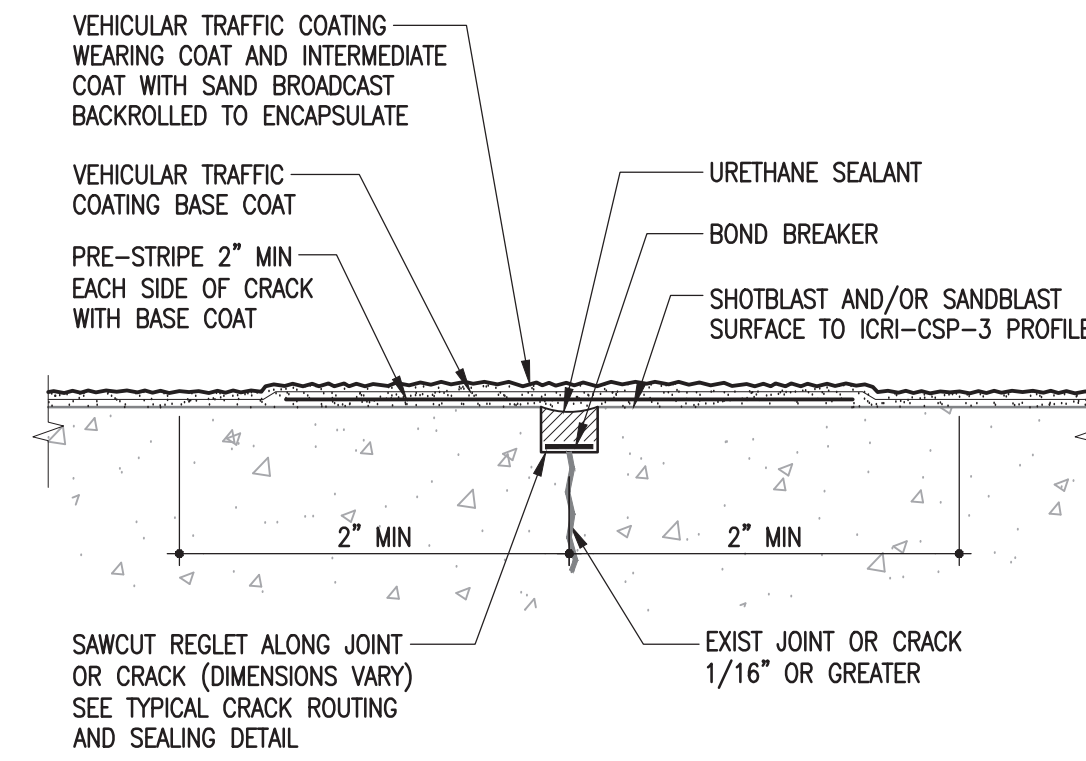
2 DETAIL AT JOINT OR CRACKS (1/16" OR GREATER) - S6.1 N.T.S. (VEHICULAR TRAFFIC COATING)
