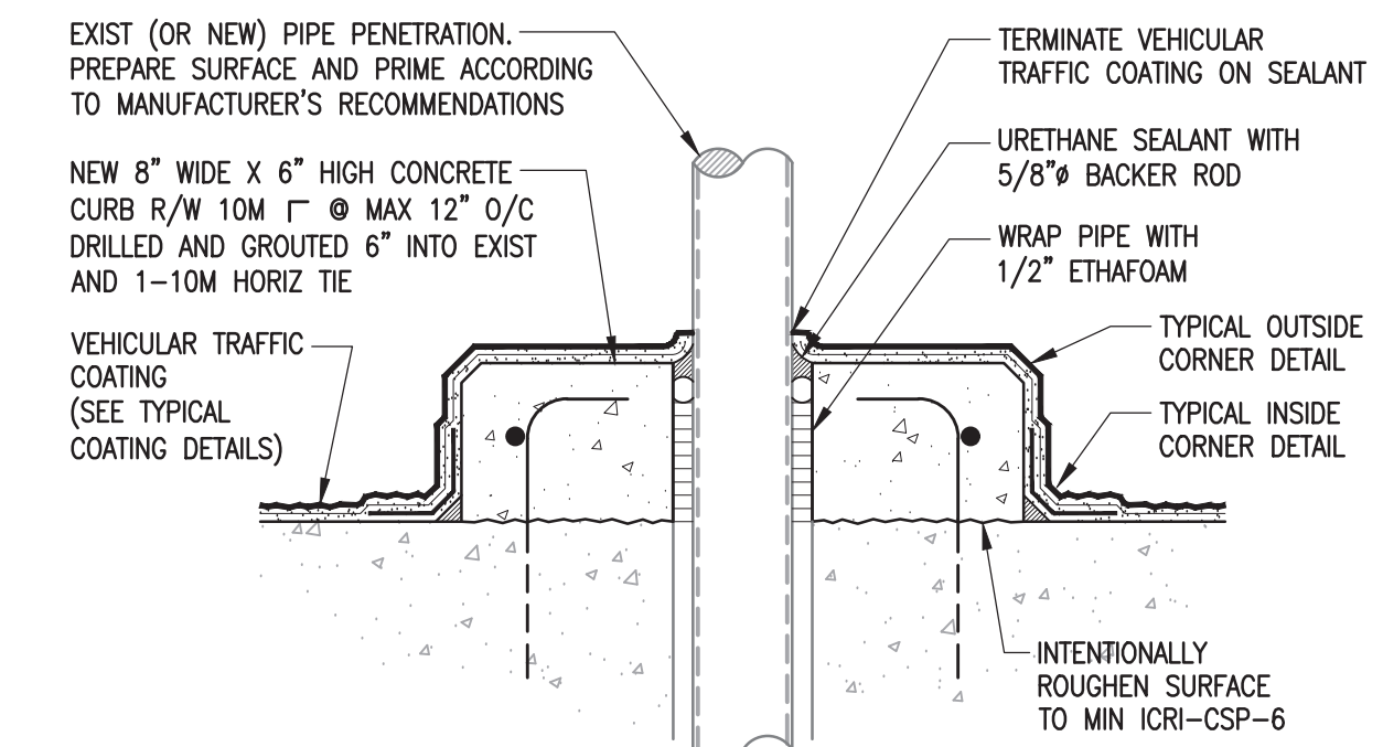
7 DETAIL AT PIPE PENETRATION - S6.1 N.T.S. (VEHICULAR TRAFFIC COATING)
