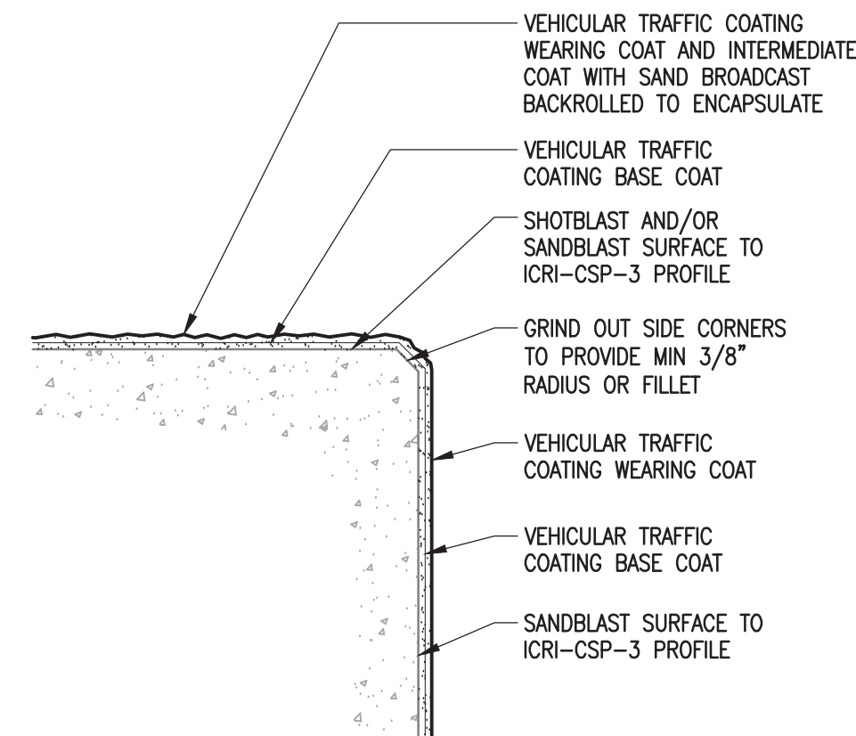
4 DETAIL AT OUTSIDE CORNER - S6.1 N.T.S. (VEHICULAR TRAFFIC COATING)
