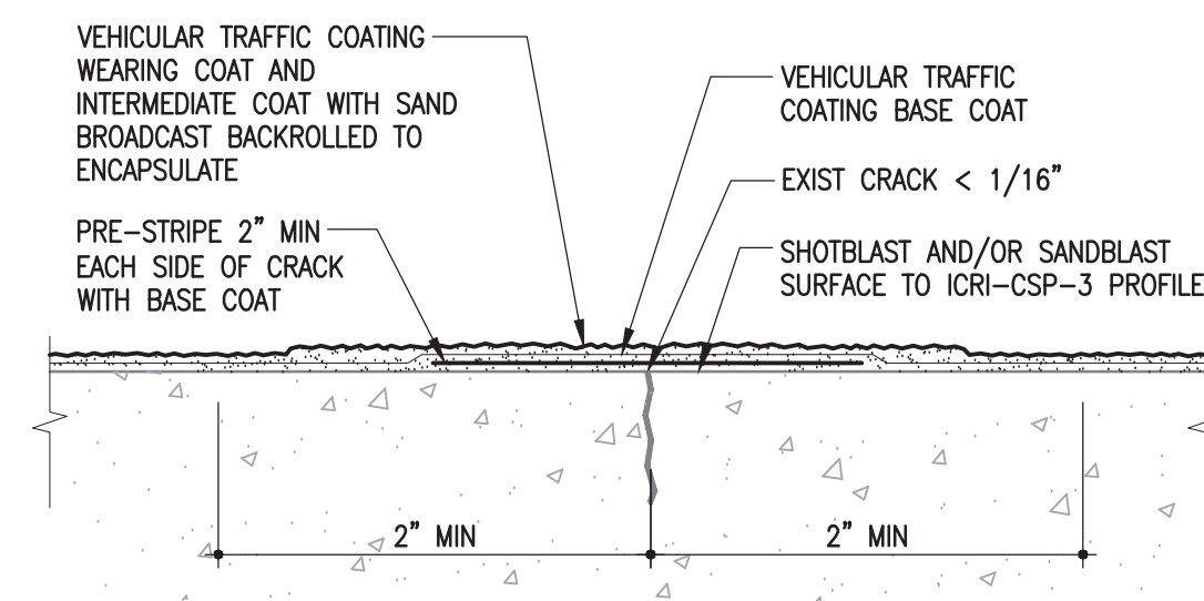
1 DETAIL AT CRACKS (< 1/16") - S6.1 N.T.S. (VEHICULAR TRAFFIC COATING)
