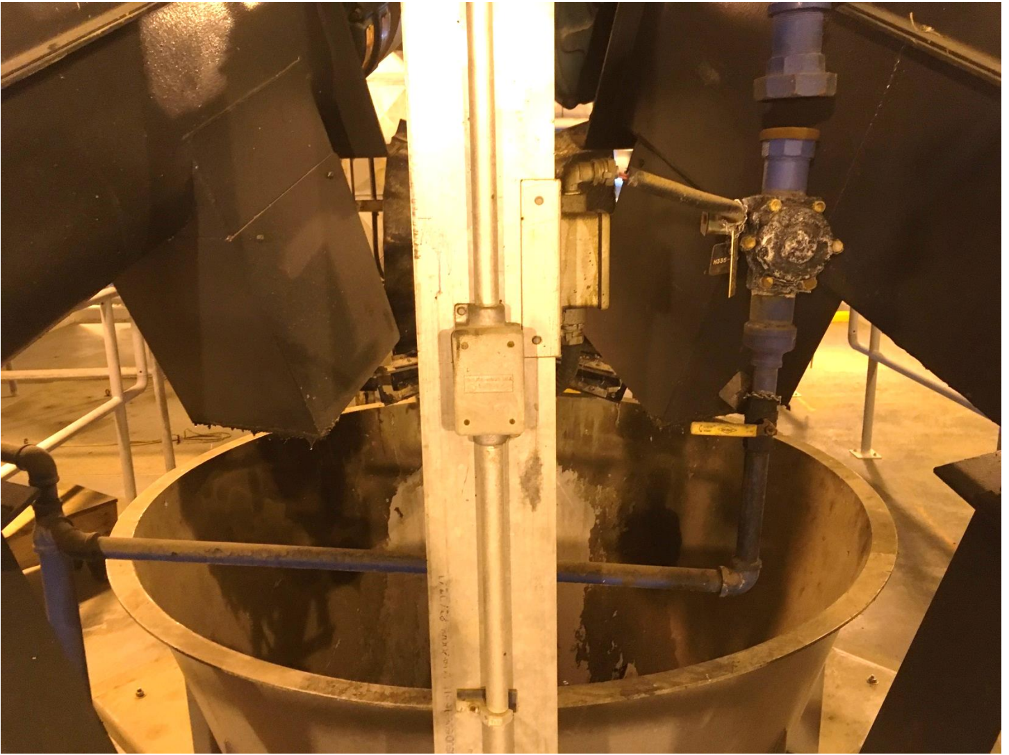
Figure 6: Flushing water pipe and Solenoid Valve
