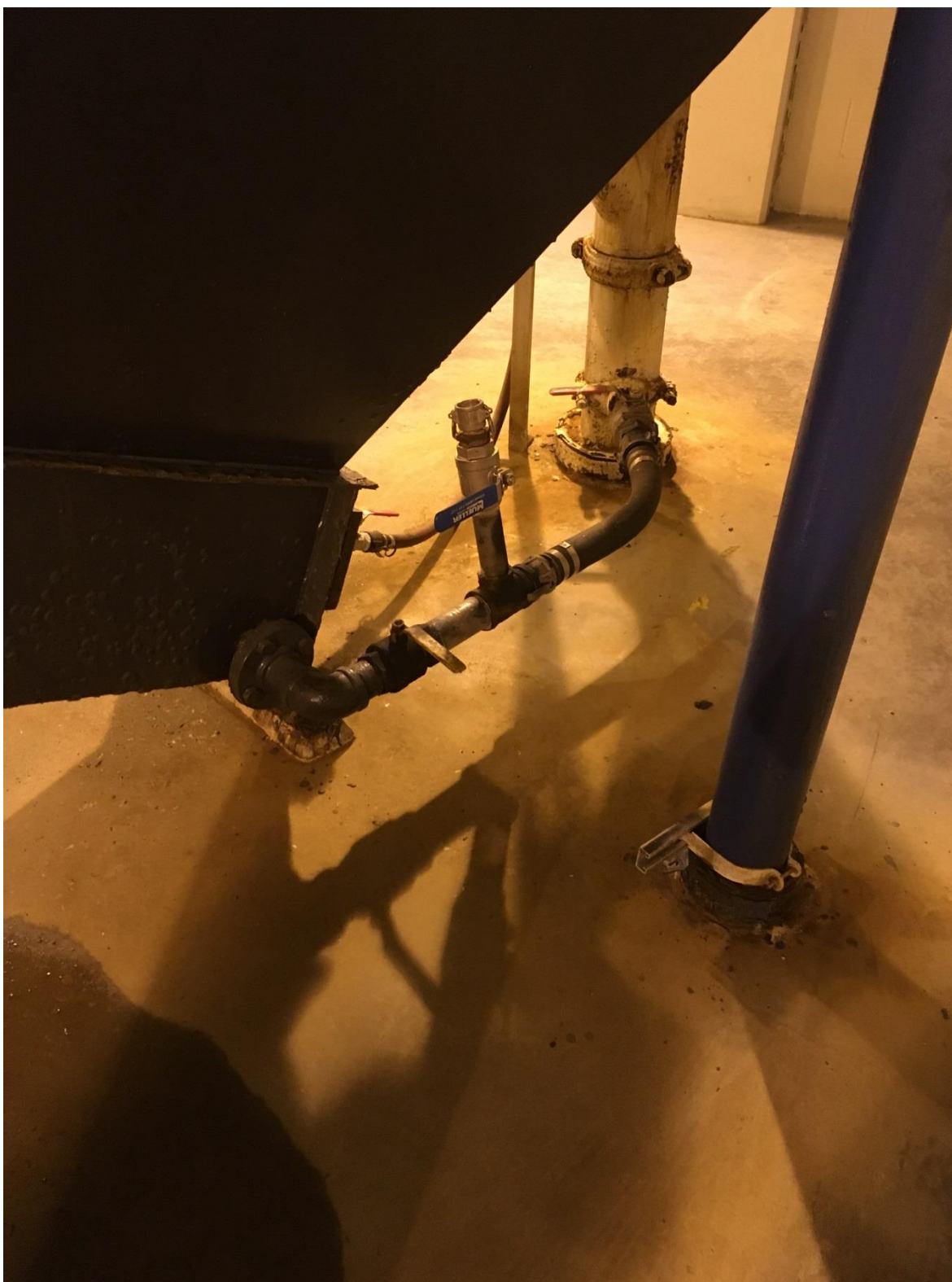
Figure 4: Grit Classifier Drain Piping
