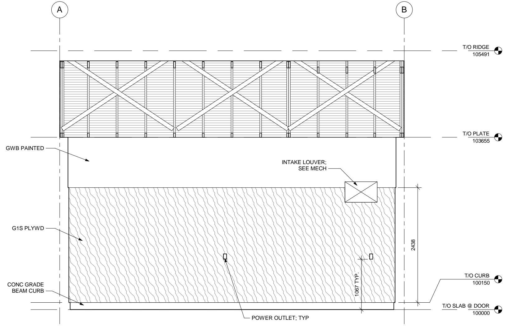
2 INT ELEVATION - GARAGE - B 1 : 50
