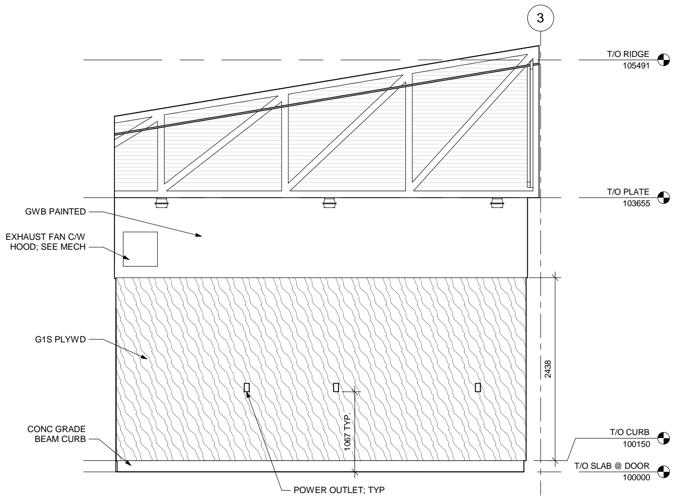
1 INT ELEVATION - GARAGE - A 1 : 50
