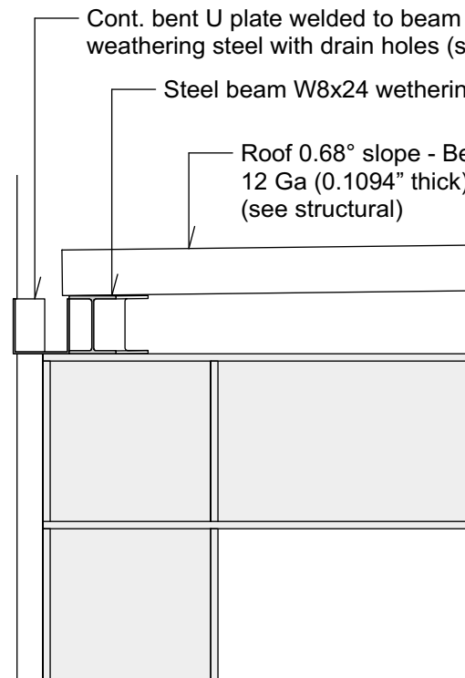
1 Detail 1 (elevation) Scale: 1/2" = 1'-0"
