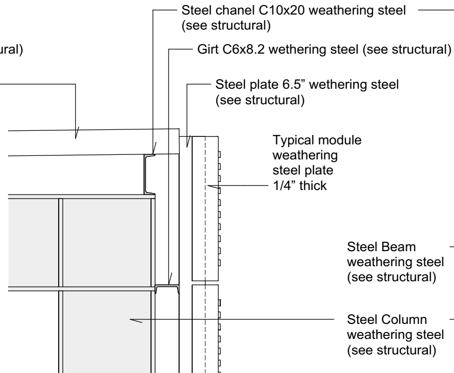
2 Detail 2 (elevation) Scale: 1/2" = 1'-0"
