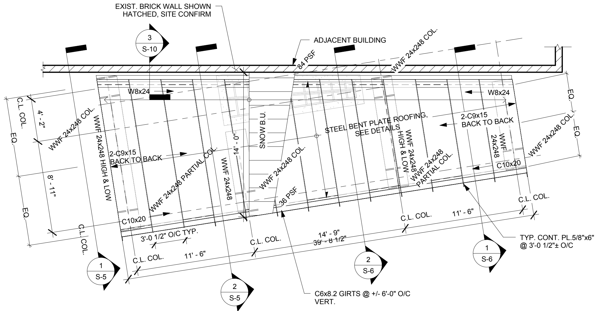
1 ROOF FRAMING PLAN 3/16" = 1'-0"
