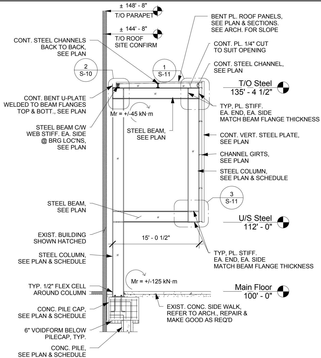
1 SECTION 1/8" = 1'-0"
