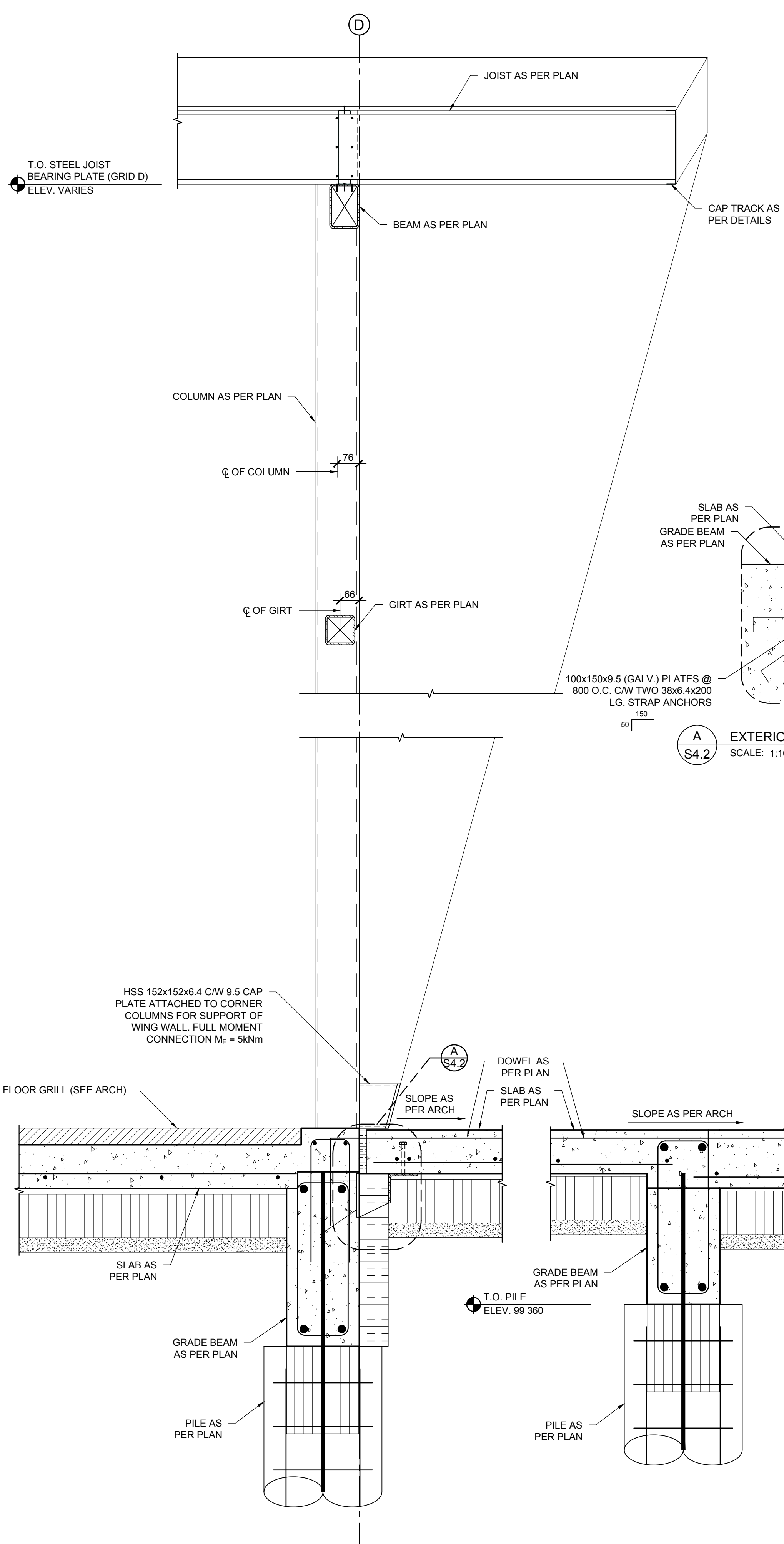
2 FULL HEIGHT SECTION SCALE: 1:10
