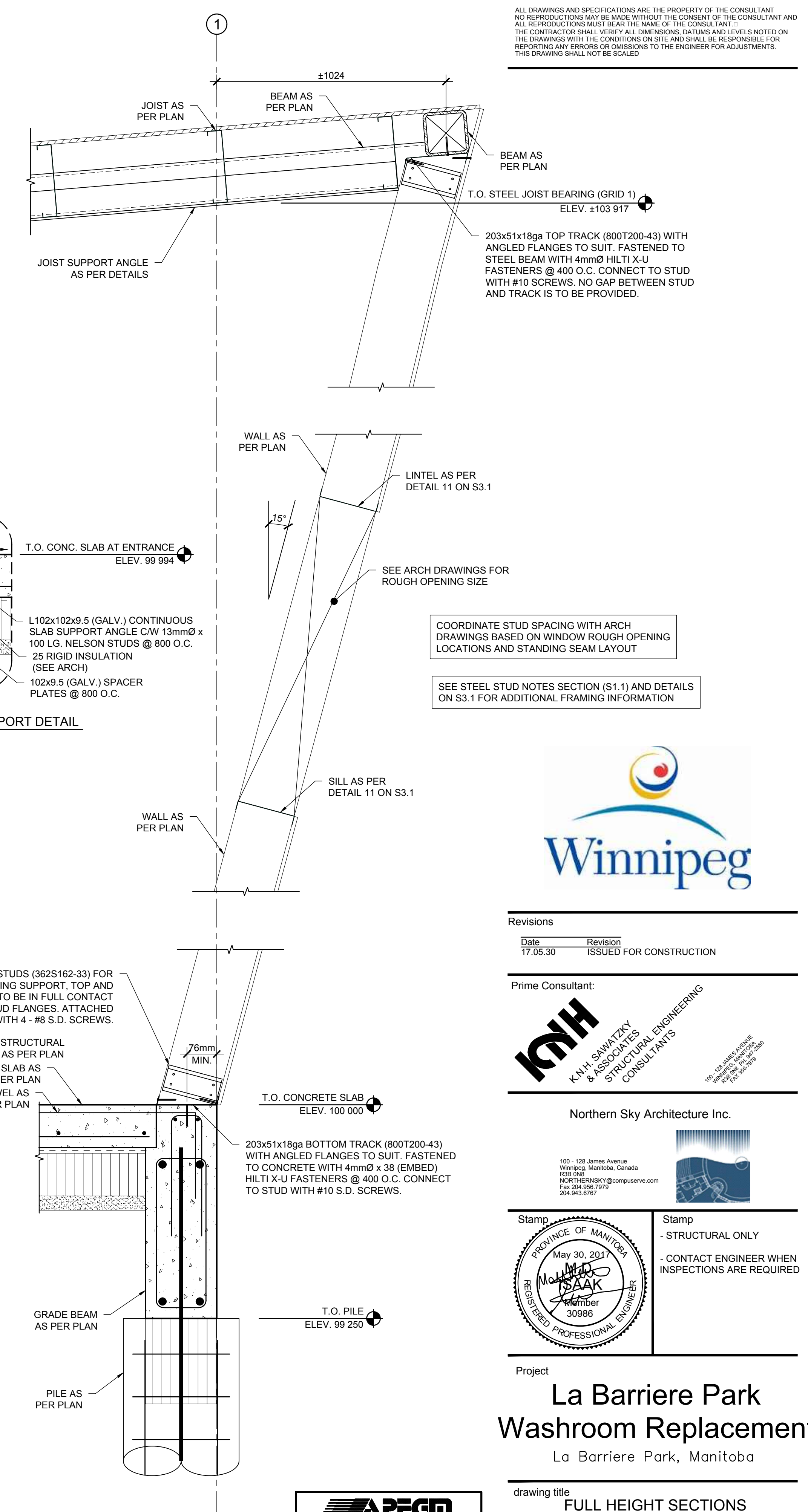
3 FULL HEIGHT SECTION SCALE: 1:10
