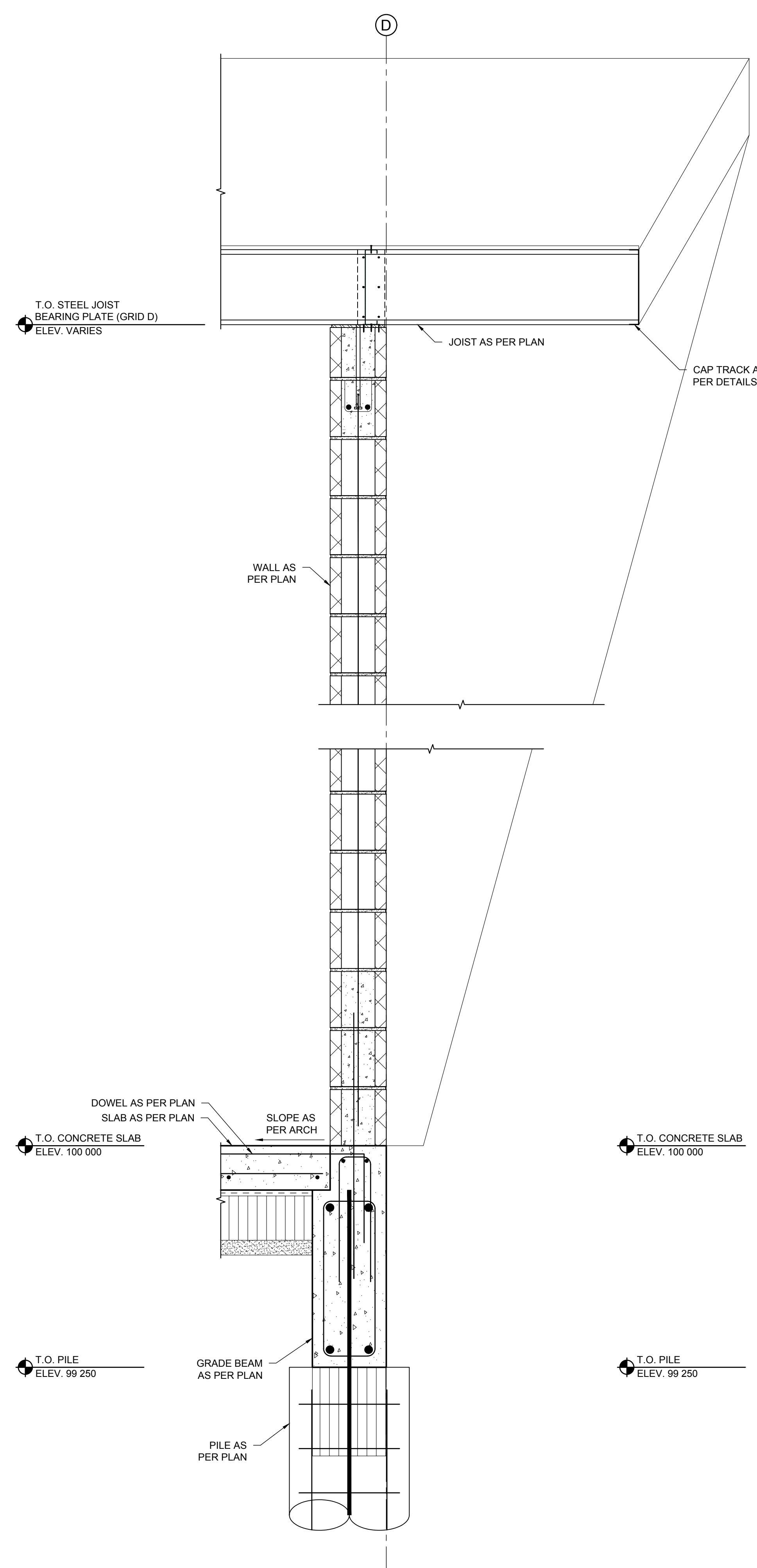
1 FULL HEIGHT SECTION SCALE: 1:10
