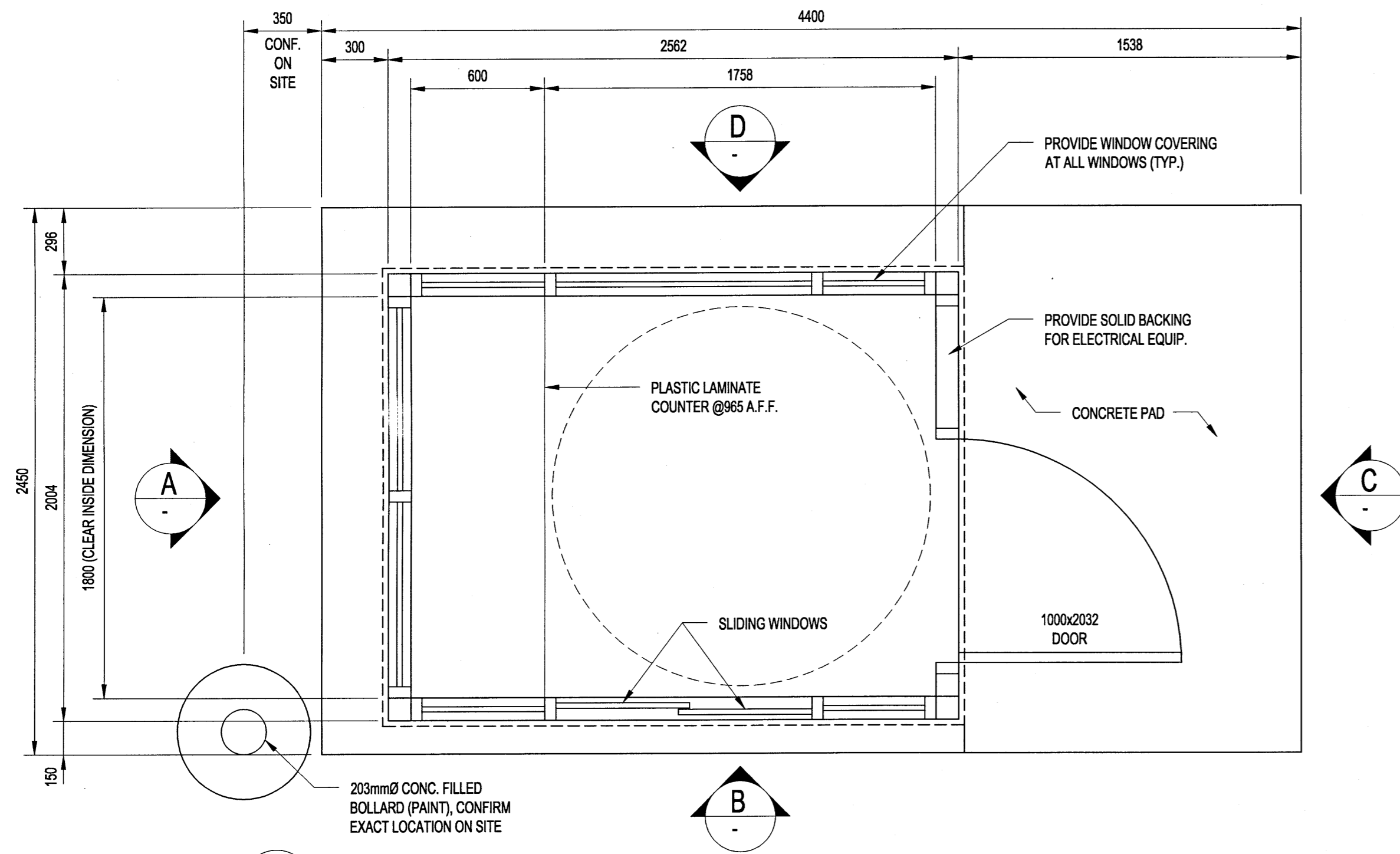
1 B01 KIOSK FLOOR PLAN SCALE: 1:20
